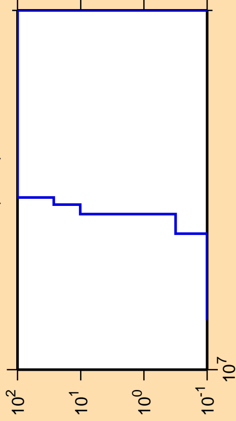
\Delta\sigma/\sigma vs. E for ^{150}\text{Pr}(n,nd)
