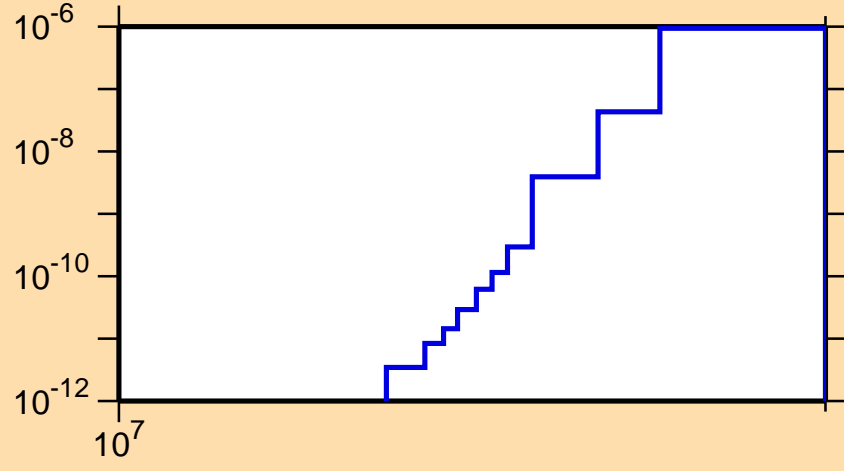
\sigma vs. E for ^{150}\text{Pr}(n,2n\alpha)
