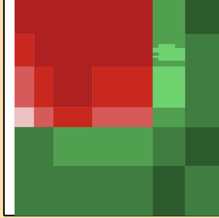
\Delta\sigma/\sigma vs. E for ^{150}\text{Pr}(n,2n)
