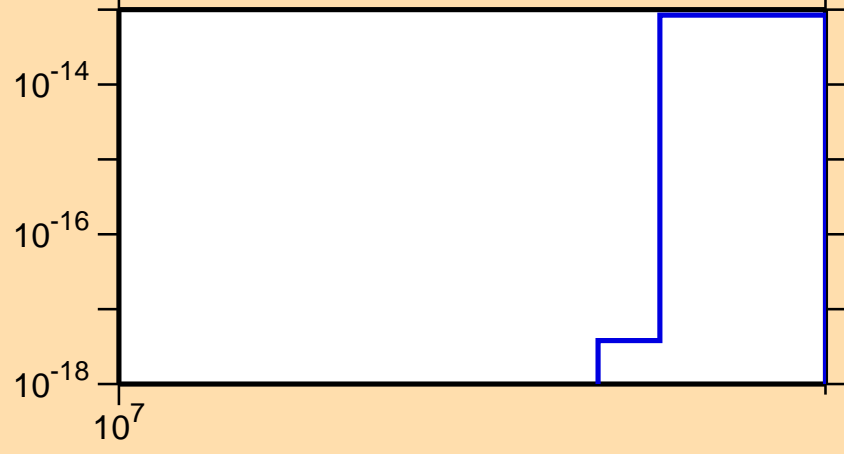
\sigma vs. E for ^{150}\text{Pr}(n,3n\alpha)
