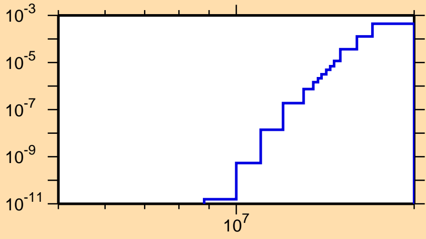
\sigma vs. E for ^{150}\text{Pr}(n,\alpha)
