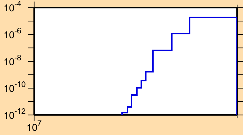
\sigma vs. E for ^{150}\text{Pr}(n,nd)
