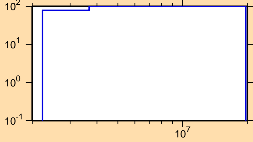
\Delta\sigma/\sigma vs. E for ^{150}\text{Pr}(n,n_1)
