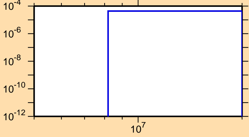
\sigma vs. E for ^{150}\text{Pr}(n,t)
