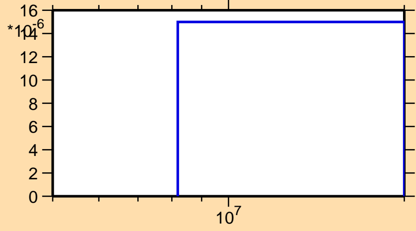
\sigma vs. E for ^{150}\text{Pr}(n,\alpha)
