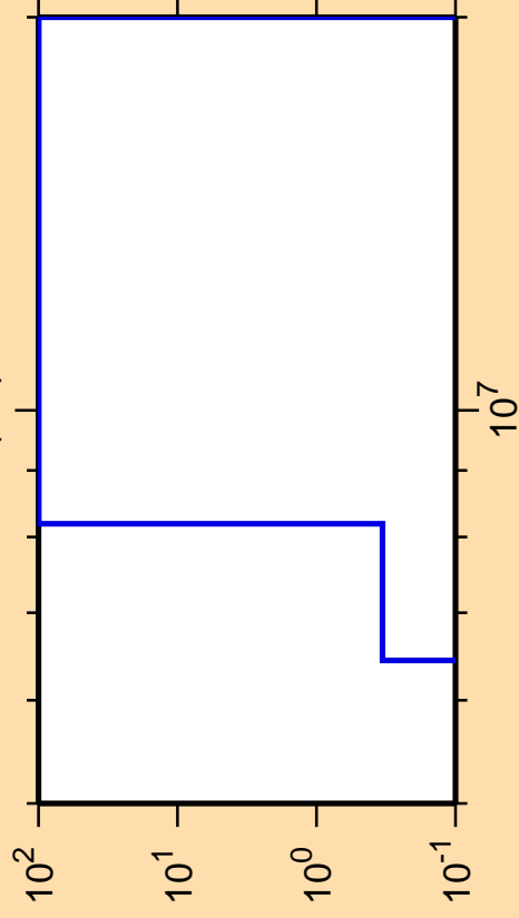
\Delta\sigma/\sigma vs. E for ^{150}\text{Pr}(n,t)
