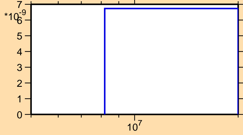
\sigma vs. E for ^{150}\text{Pr}(n,2np)
