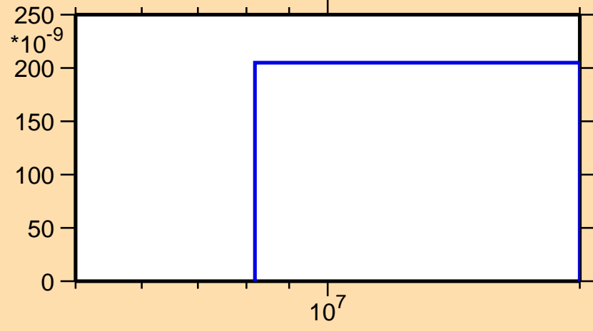
\sigma vs. E for ^{150}\text{Pr}(n,\text{nd})
