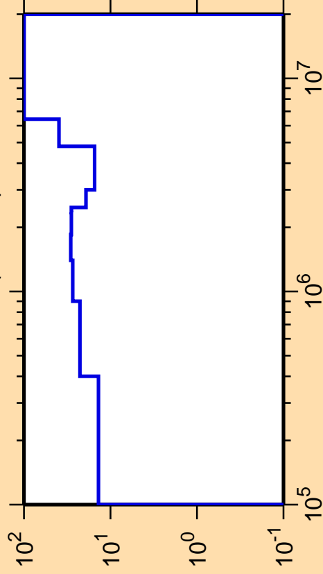
\Delta\sigma/\sigma vs. E for ^{150}\text{Pr}(n,\text{inel.})
