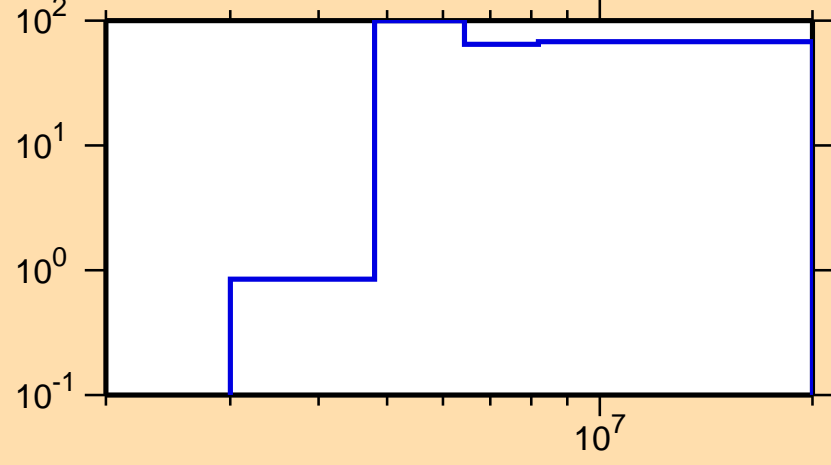
\Delta\sigma/\sigma vs. E for ^{150}\text{Pr}(n,p)
