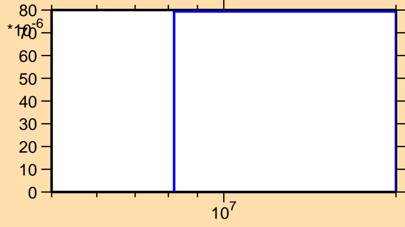
\sigma vs. E for ^{150}\text{Pr}(n,d)
