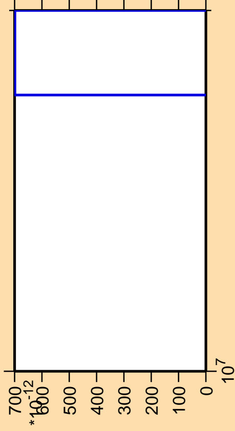
\Delta\sigma/\sigma vs. E for ^{151}\text{Pr}(\text{mt } 42)
