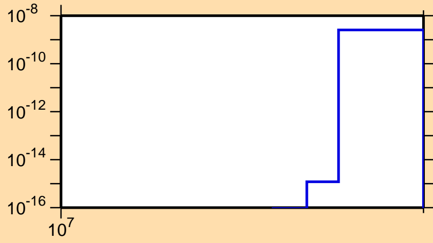
\sigma vs. E for ^{151}\text{Pr}(n,2np)
