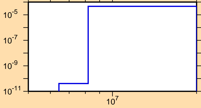
\sigma vs. E for ^{151}\text{Pr}(n,\alpha)
