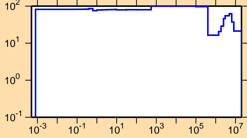
\Delta\sigma/\sigma vs. E for ^{151}\text{Pr}(n,\text{el.})
