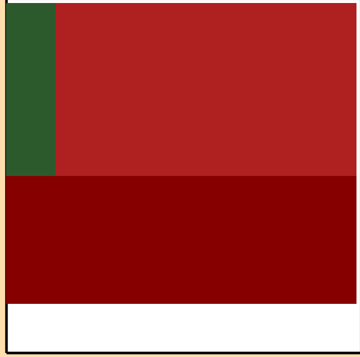
\Delta\sigma/\sigma vs. E for ^{152}\text{Pr}(n,p)
