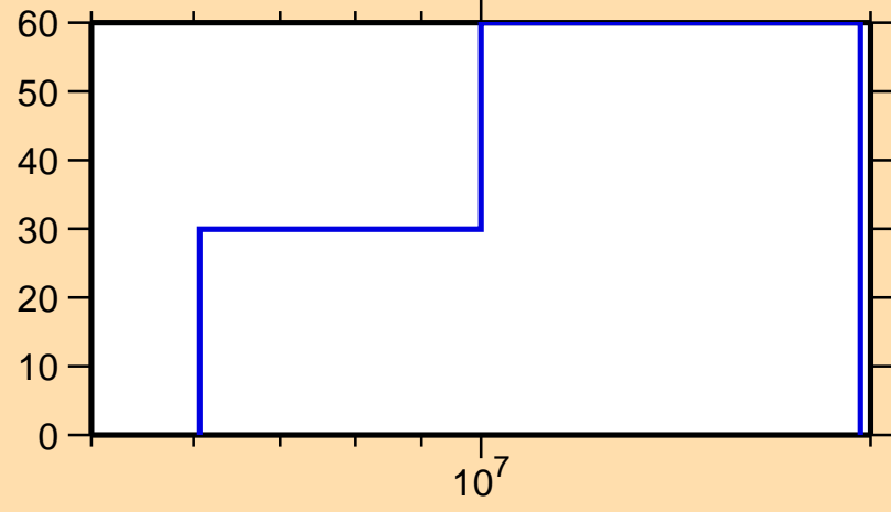
\Delta\sigma/\sigma vs. E for ^{152}\text{Pr}(n,ncont.)
