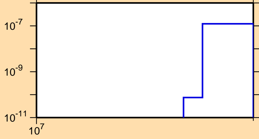
\sigma vs. E for ^{153}\text{Pr}(n,\text{nd})
