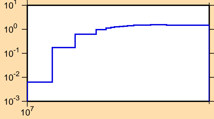
\sigma vs. E for ^{154}\text{Pr}(n,3n)
