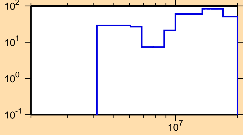
\Delta\sigma/\sigma vs. E for ^{154}\text{Pr}(n,2n)
