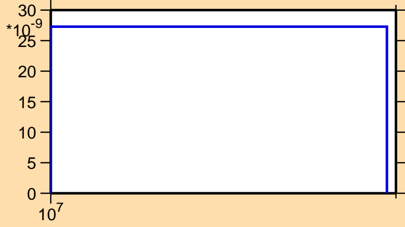
\sigma vs. E for ^{154}\text{Pr}(n,nt)
