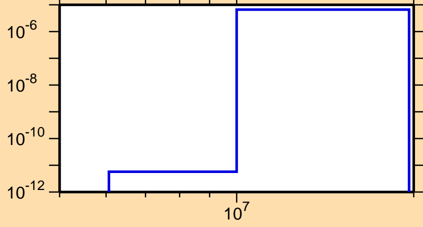
\sigma vs. E for ^{154}\text{Pr}(n,\alpha)
