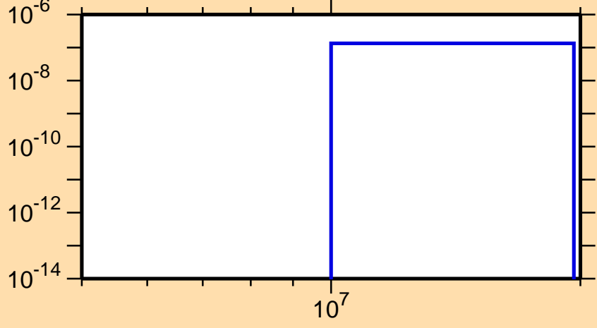
\sigma vs. E for ^{154}\text{Pr}(n,\alpha)
