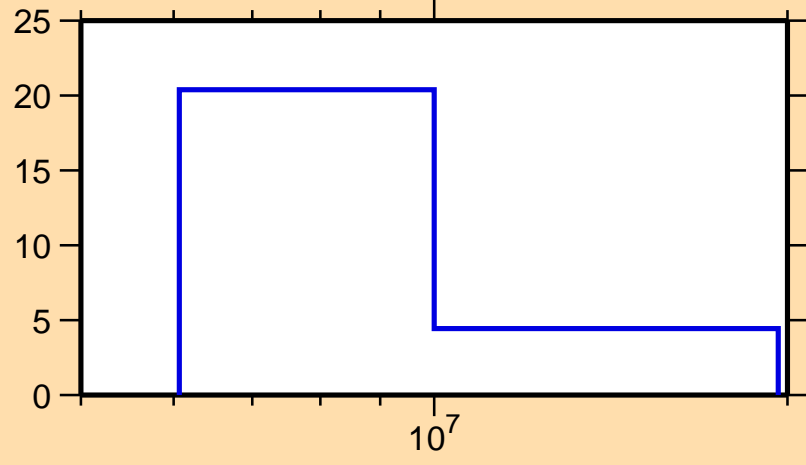
\Delta\sigma/\sigma vs. E for ^{154}\text{Pr}(n,el.)
