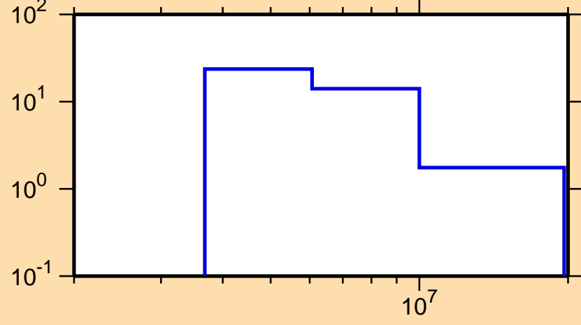
\Delta\sigma/\sigma vs. E for ^{154}\text{Pr}(n,\text{tot.})
