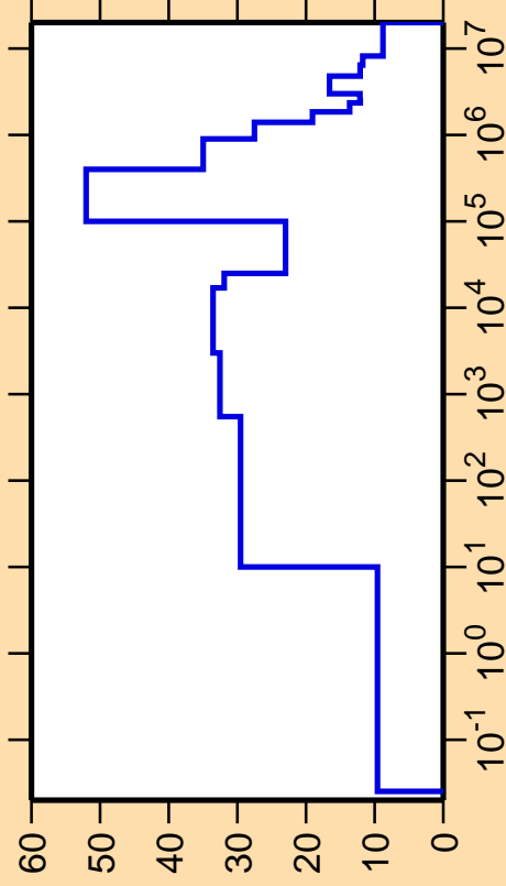
\Delta\sigma/\sigma vs. E for ^{154}\text{Pr}(n,\text{nonel.})
