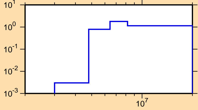
\sigma vs. E for ^{154}\text{Pr}(n,2n)
