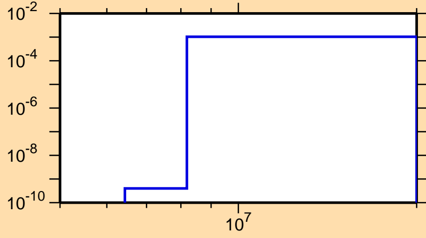
\sigma vs. E for ^{154}\text{Pr}(n,p)
