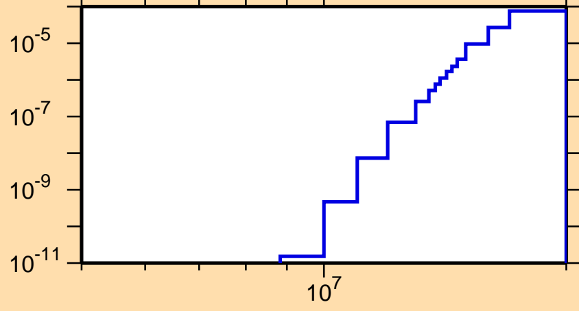
\sigma vs. E for ^{155}\text{Pr}(n,\alpha)
