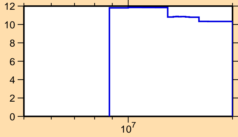
\Delta\sigma/\sigma vs. E for ^{155}\text{Pr}(n,el.)
