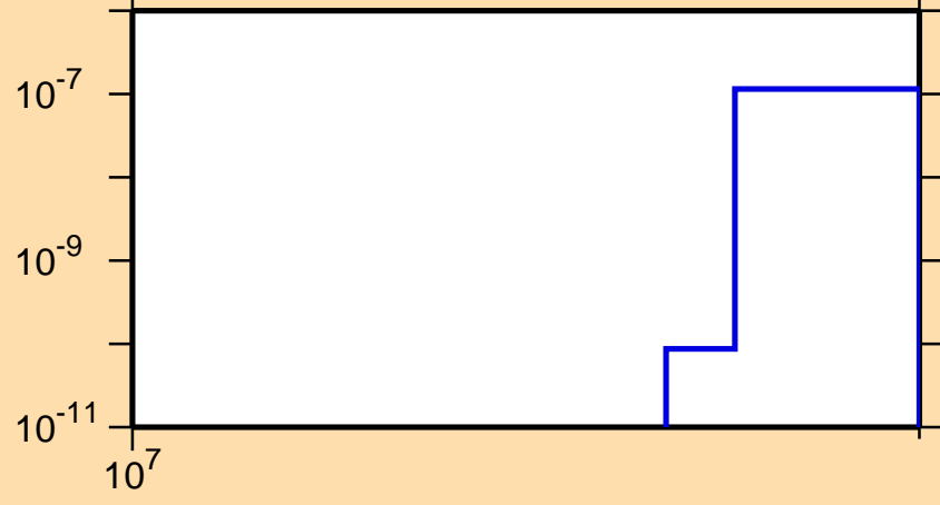
\sigma vs. E for ^{155}\text{Pr}(n,\text{nd})
