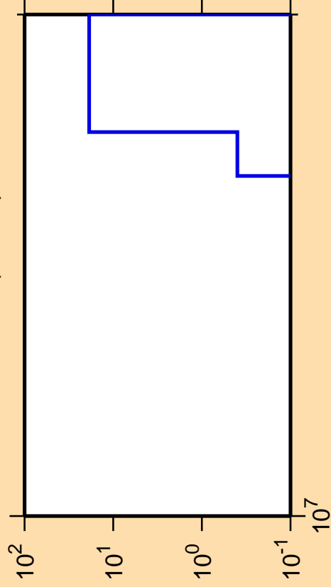
\Delta\sigma/\sigma vs. E for ^{228}\text{Pu} (mt 34)
