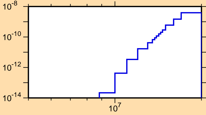
\sigma vs. E for ^{228}\text{Pu}(\text{mt 45})
