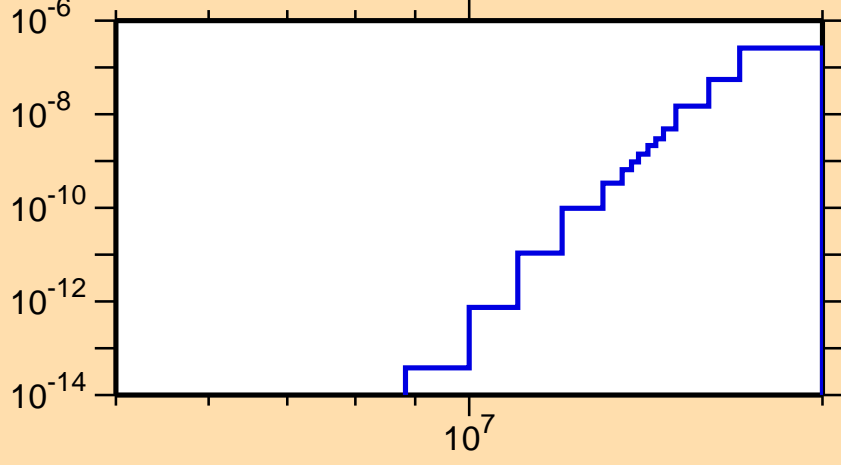
\sigma vs. E for ^{228}\text{Pu}(n,\text{He3})
