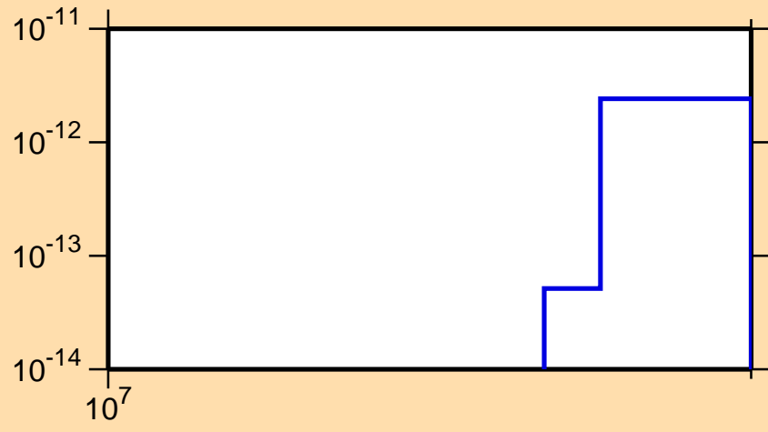
\sigma vs. E for ^{228}\text{Pu} (mt 34)
