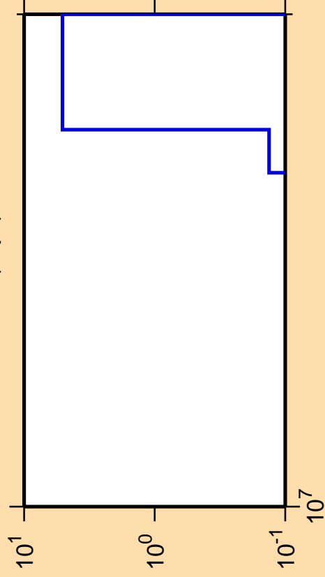
\Delta\sigma/\sigma vs. E for ^{228}\text{Pu}(n,\text{pt})
