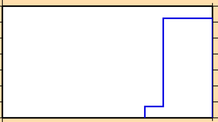
\sigma vs. E for ^{228}\text{Pu}(n,\text{pd})
