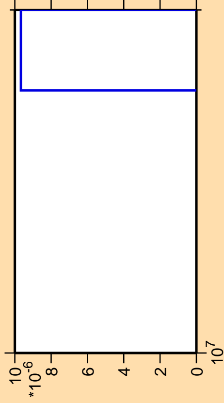
\Delta\sigma/\sigma vs. E for ^{228}\text{Pu} (mt 42)
