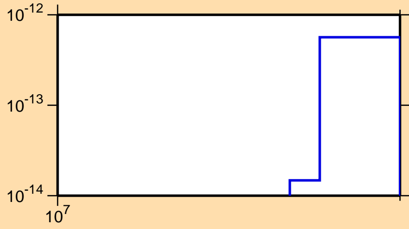
\sigma vs. E for ^{228}\text{Pu}(n,\text{pt})
