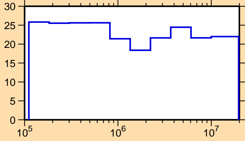
\Delta\sigma/\sigma vs. E for ^{228}\text{Pu}(n,nonel.)
