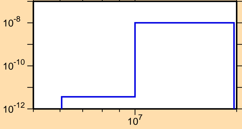
\sigma vs. E for ^{228}\text{Pu}(n,p\alpha)
