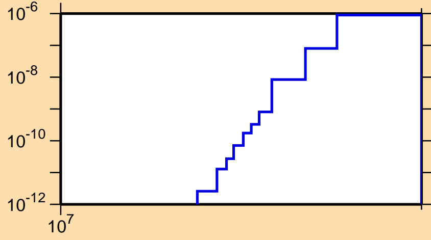
\sigma vs. E for ^{229}\text{Pu}(n,\text{nd})
