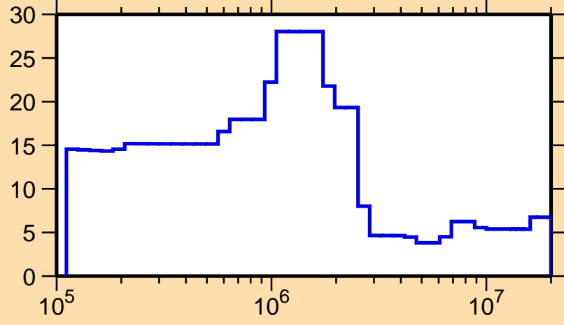
\Delta\sigma/\sigma vs. E for ^{229}\text{Pu}(n,n\text{onel.})
