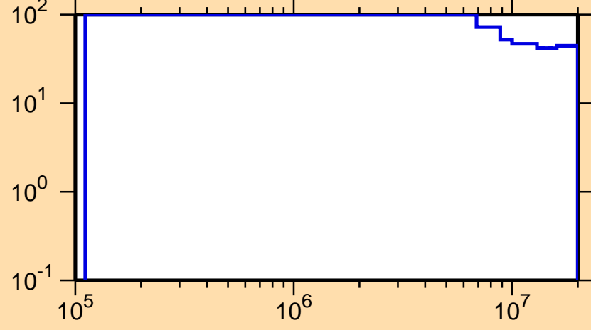
\Delta\sigma/\sigma vs. E for ^{229}\text{Pu}(n,n\text{cont.})
