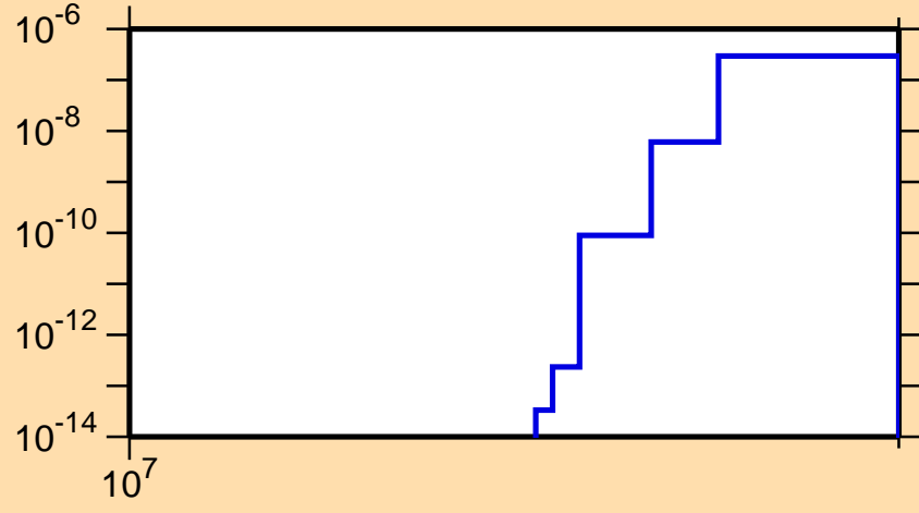
\sigma vs. E for ^{230}\text{Pu}(n,2np)
