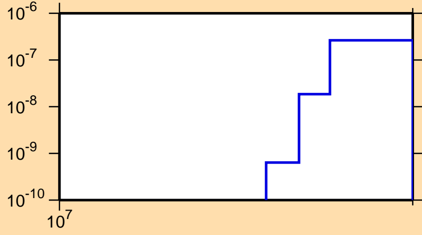
\sigma vs. E for ^{230}\text{Pu}(n,3n)
