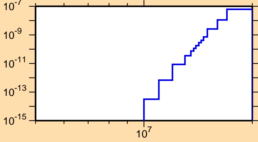
\sigma vs. E for ^{230}\text{Pu}(n,\text{He}3)
