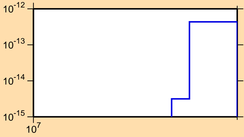
\sigma vs. E for ^{230}\text{Pu} (mt 34)
