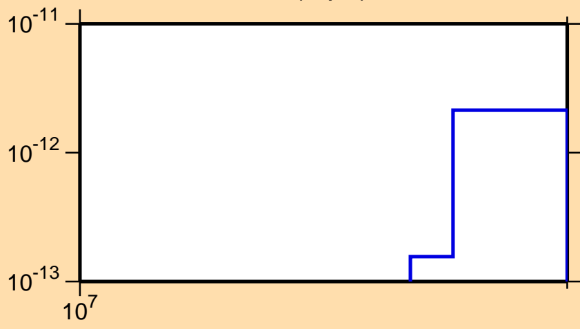
\sigma vs. E for ^{230}\text{Pu}(n,\text{pd})
