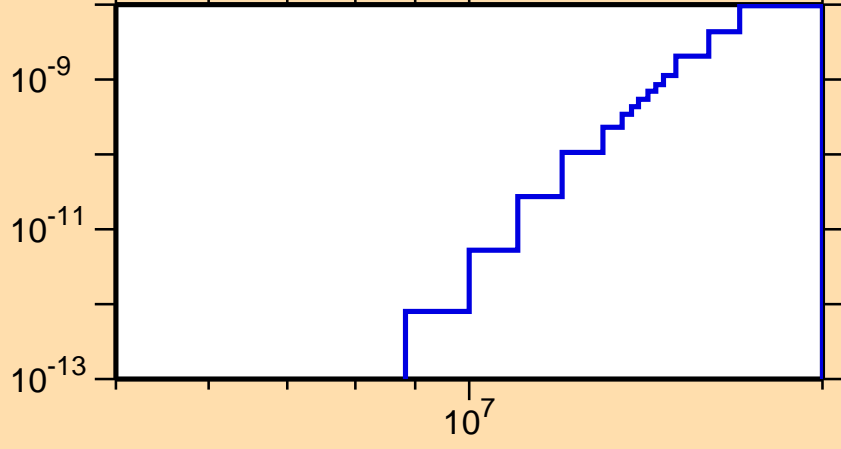
\sigma vs. E for ^{230}\text{Pu}(n,p\alpha)
