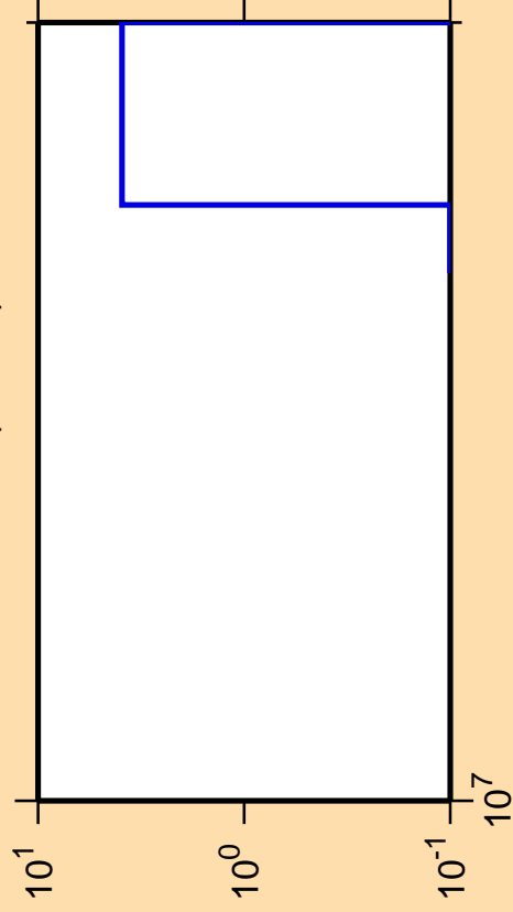
\Delta\sigma/\sigma vs. E for ^{230}\text{Pu} (mt 34)
