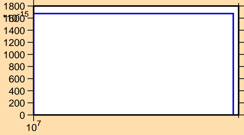
\sigma vs. E for ^{230}\text{Pu}(\text{mt117})
