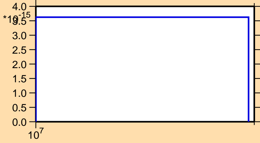
\sigma vs. E for ^{230}\text{Pu} (mt 34)
