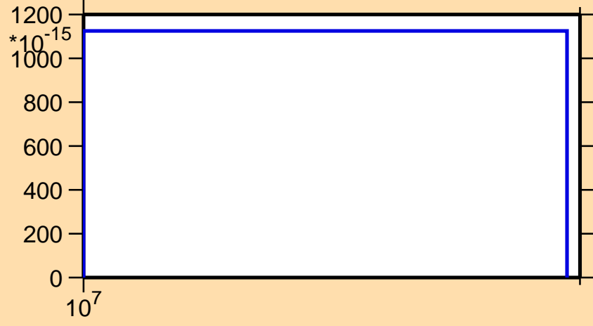
\sigma vs. E for ^{230}\text{Pu} (mt 45)
