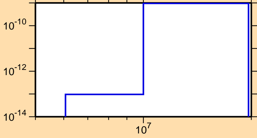
\sigma vs. E for ^{230}\text{Pu}(n,p\alpha)
