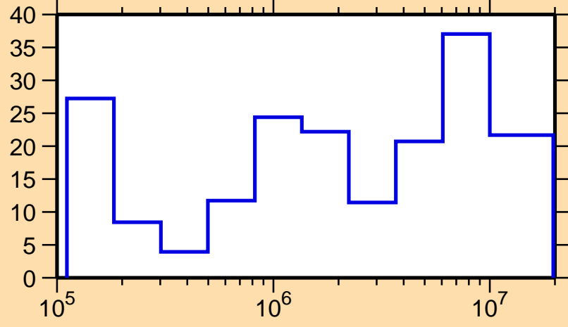
\Delta\sigma/\sigma vs. E for ^{230}\text{Pu}(n, el.)
