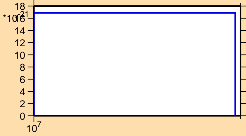
\sigma vs. E for ^{230}\text{Pu} (mt 42)
