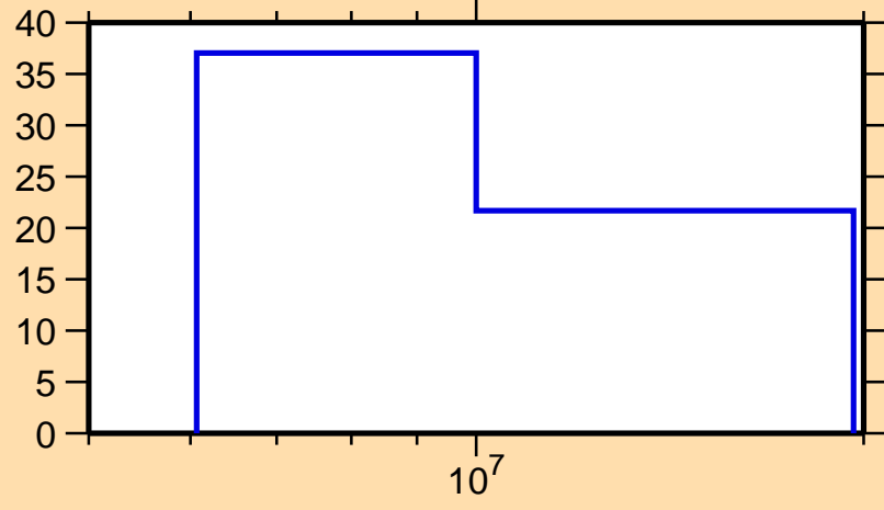
\Delta\sigma/\sigma vs. E for ^{230}\text{Pu}(n,\text{el.})
