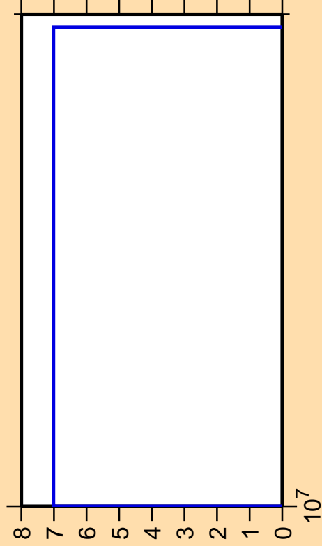
\Delta\sigma/\sigma vs. E for ^{230}\text{Pu} (mt 45)
