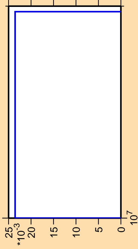
\Delta\sigma/\sigma vs. E for ^{230}\text{Pu}(n,\text{pd})
