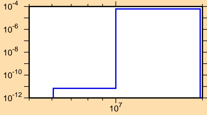
\sigma vs. E for ^{230}\text{Pu}(n,t)
