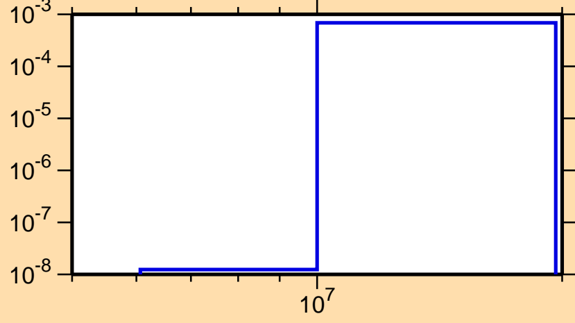
\sigma vs. E for ^{230}\text{Pu}(n,d)
