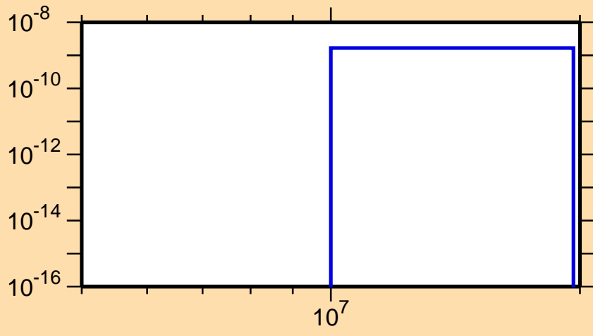
\sigma vs. E for ^{230}\text{Pu}(n,\text{He3})
