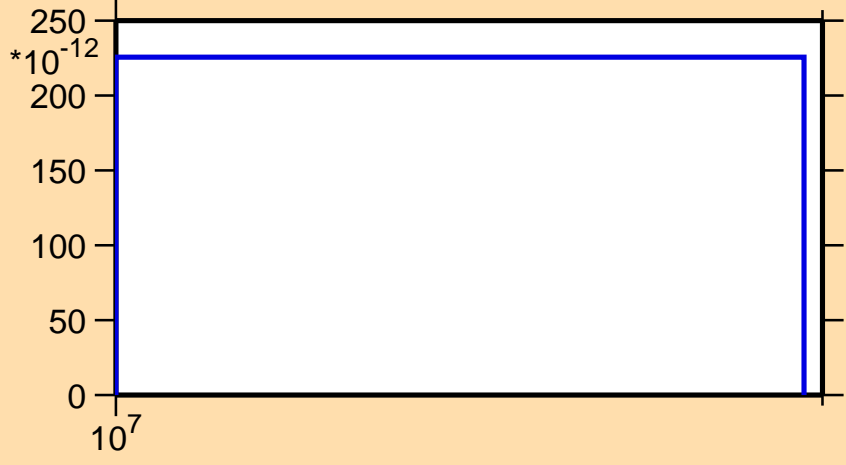
\sigma vs. E for ^{230}\text{Pu}(n,3n\alpha)
