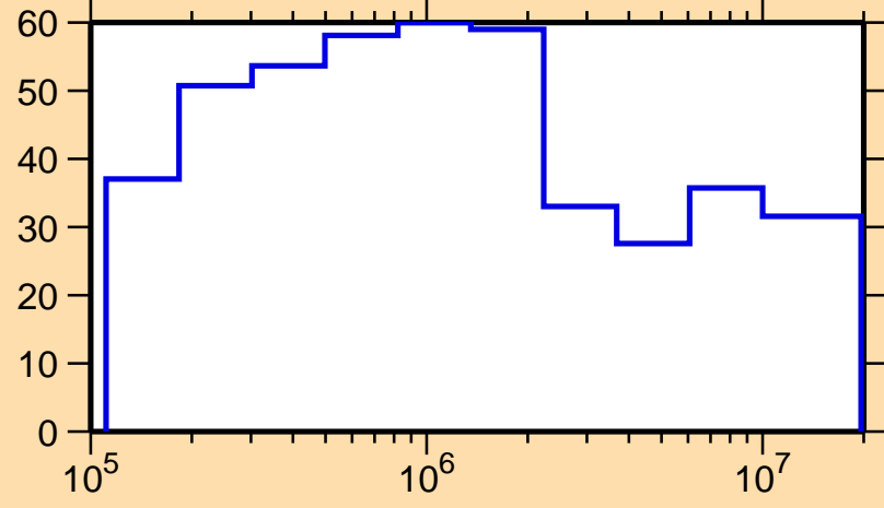
\Delta\sigma/\sigma vs. E for ^{230}\text{Pu}(n,n\text{onel.})
