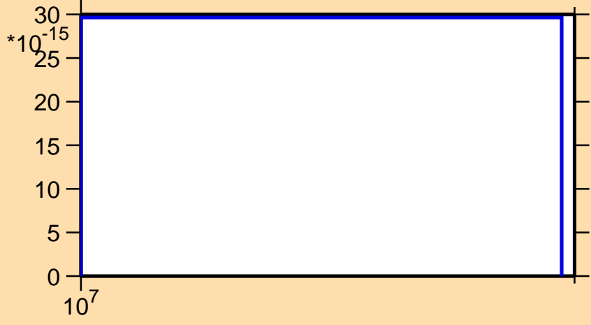
\sigma vs. E for ^{230}\text{Pu}(n,\text{pd})
