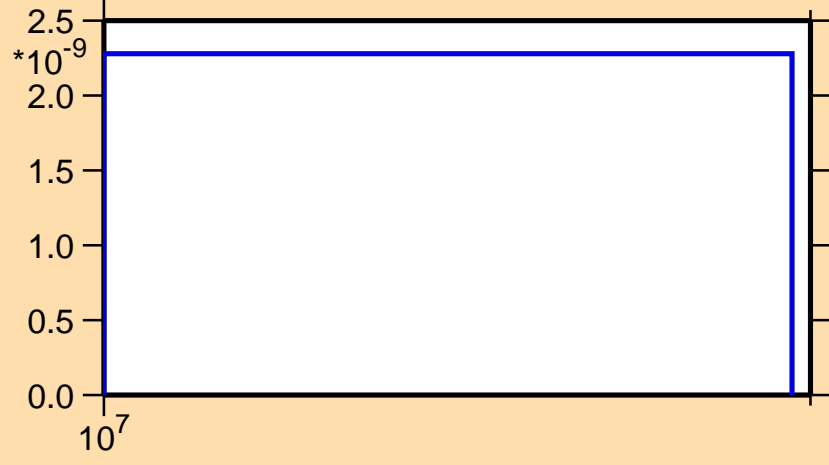
\sigma vs. E for ^{230}\text{Pu}(n,\text{nd})
