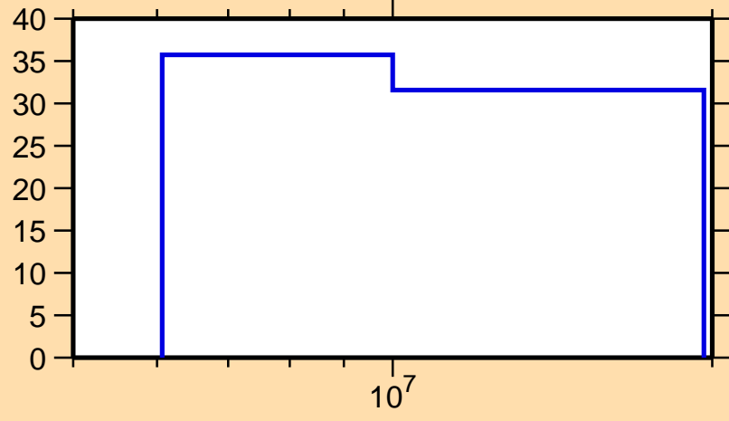
\Delta\sigma/\sigma vs. E for ^{230}\text{Pu}(n,\text{nonel.})
