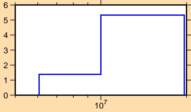
\Delta\sigma/\sigma vs. E for ^{230}\text{Pu}(n,\text{tot.})
