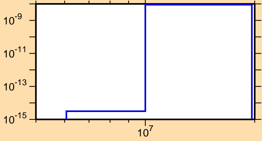
\sigma vs. E for ^{230}\text{Pu}(n,2n\alpha)
