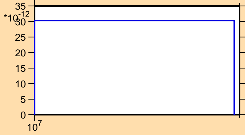
\sigma vs. E for ^{230}\text{Pu}(n,nt)
