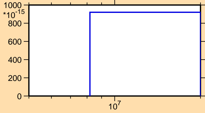
\sigma vs. E for ^{230}\text{Pu}(\text{mt } 45)
