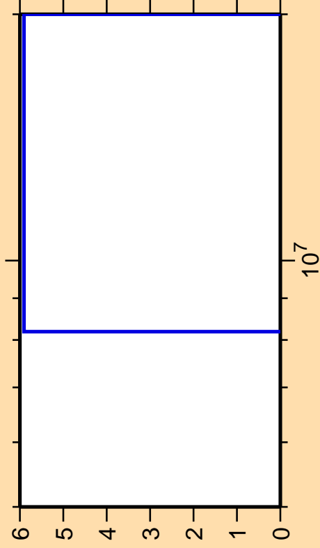
\Delta\sigma/\sigma vs. E for ^{230}\text{Pu}(n,t)
