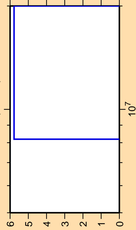
\Delta\sigma/\sigma vs. E for ^{230}\text{Pu}(\text{mt } 45)
