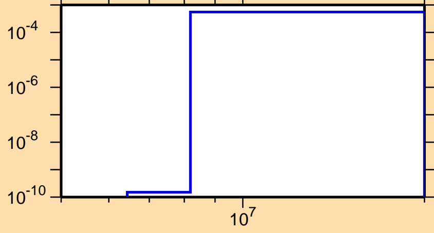
\sigma vs. E for ^{230}\text{Pu}(n,d)
