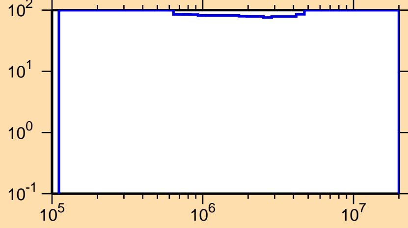
\Delta\sigma/\sigma vs. E for ^{231}\text{Pu}(n,ncont.)
