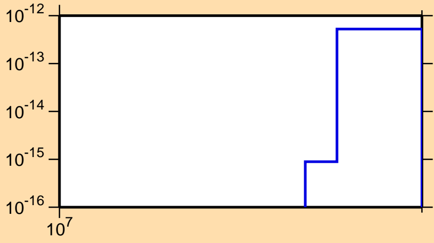
\sigma vs. E for ^{231}\text{Pu}(n,3n\alpha)
