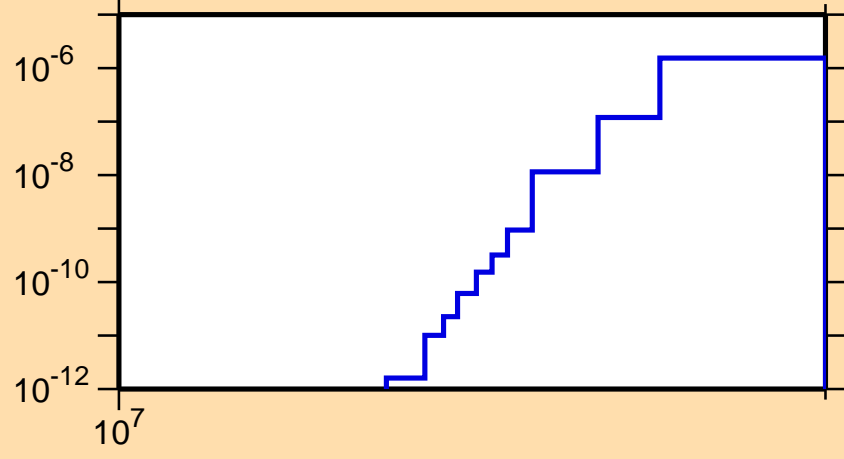
\sigma vs. E for ^{231}\text{Pu}(n,\text{nd})
