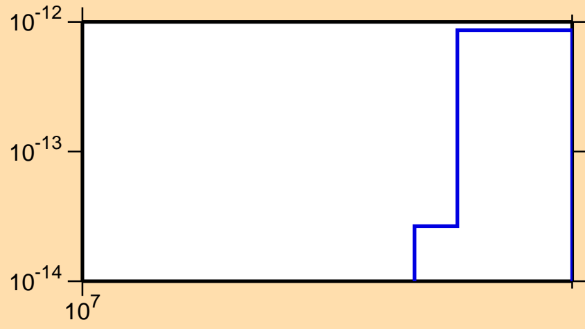
\sigma vs. E for ^{231}\text{Pu}(n,\text{pt})
