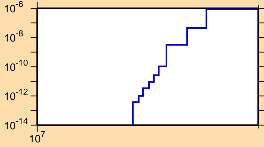
\sigma vs. E for ^{231}\text{Pu}(n,2np)
