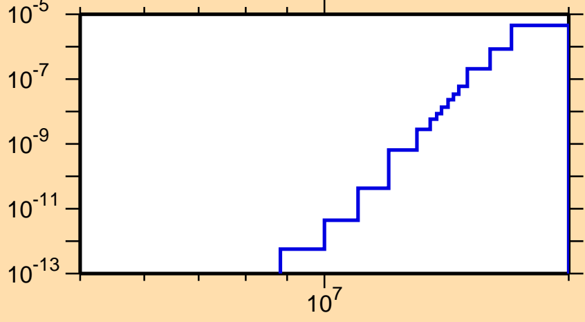
\sigma vs. E for ^{231}\text{Pu}(n,2n\alpha)
