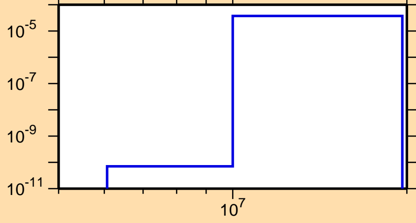
\sigma vs. E for ^{231}\text{Pu}(n,np)
