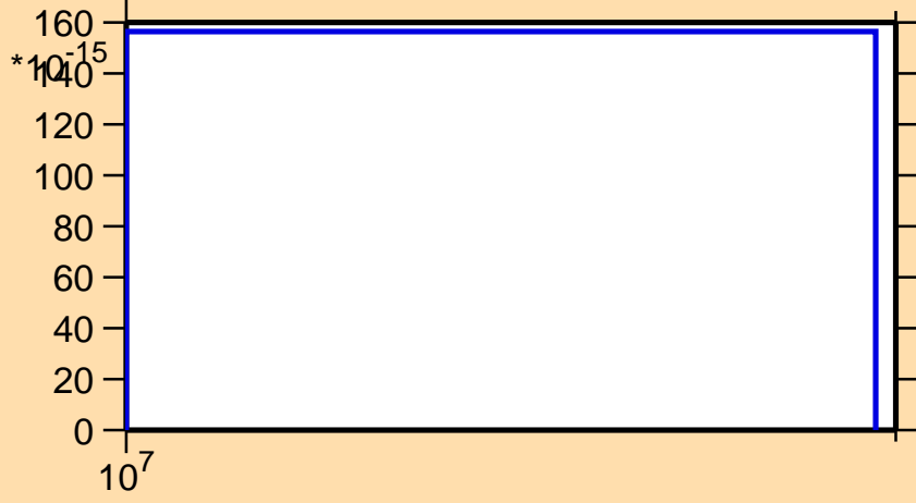
\sigma vs. E for ^{231}\text{Pu} (mt 34)
