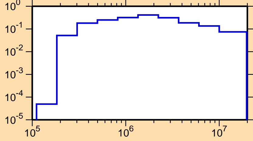
\sigma vs. E for ^{231}\text{Pu}(n,\text{inel.})
