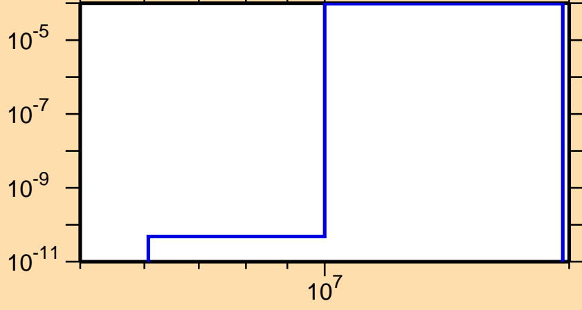
\sigma vs. E for ^{231}\text{Pu}(n,t)
