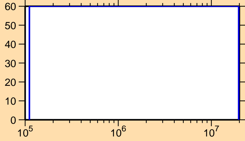
\Delta\sigma/\sigma vs. E for ^{231}\text{Pu}(n,n\text{cont.})
