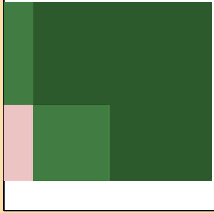
\Delta\sigma/\sigma vs. E for ^{231}\text{Pu}(n,\text{tot.})
