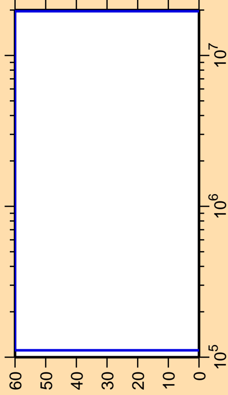
\Delta\sigma/\sigma vs. E for ^{231}\text{Pu}(n,\text{ncont.})
