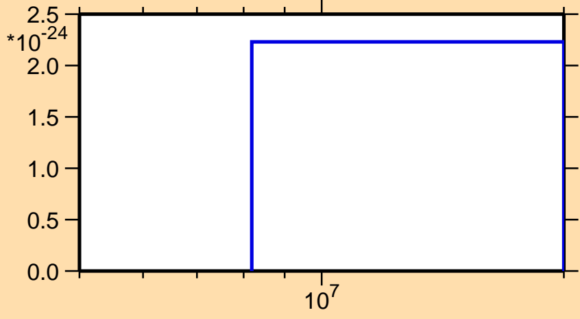
\sigma vs. E for ^{231}\text{Pu}(\text{mt } 42)
