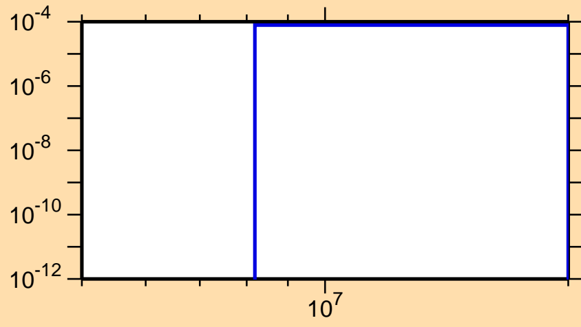
\sigma vs. E for ^{231}\text{Pu}(n,t)
