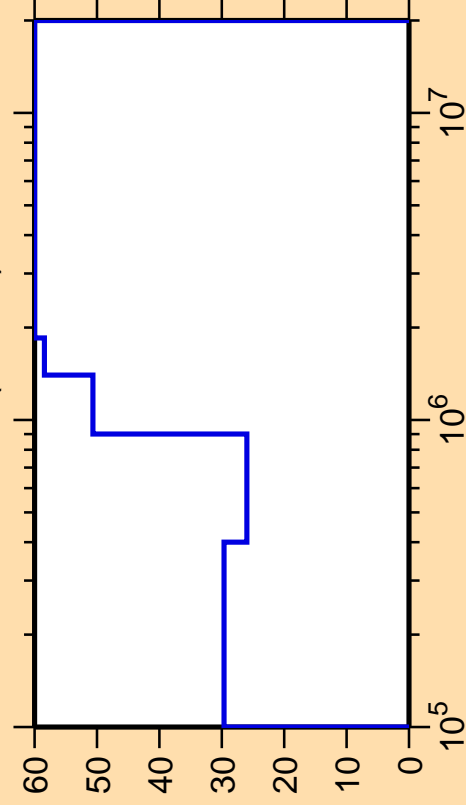
\Delta\sigma/\sigma vs. E for ^{231}\text{Pu}(n,\text{inel.})
