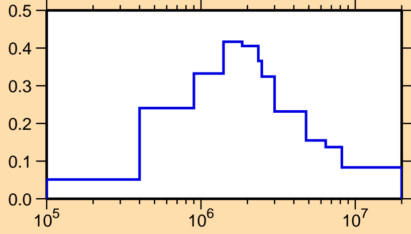
\sigma vs. E for ^{231}\text{Pu}(n,\text{inel.})
