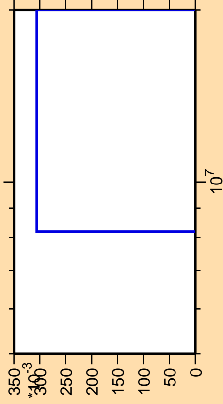
\Delta\sigma/\sigma vs. E for ^{231}\text{Pu}(\text{mt } 45)
