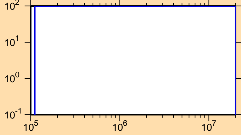
\Delta\sigma/\sigma vs. E for ^{232}\text{Pu}(n,n\text{cont.})
