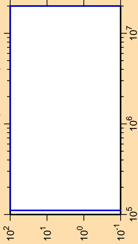
\Delta\sigma/\sigma vs. E for ^{232}\text{Pu}(n,\text{ncont.})
