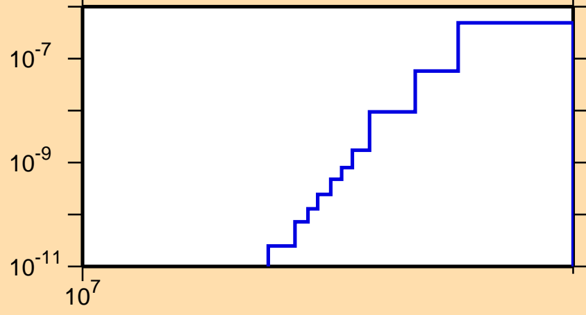
\sigma vs. E for ^{232}\text{Pu}(n,2n\alpha)
