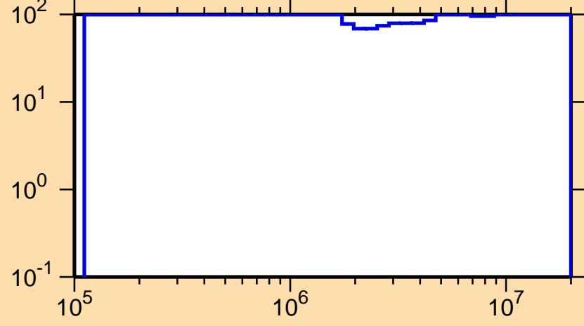
\Delta\sigma/\sigma vs. E for ^{232}\text{Pu}(n,\text{inel.})
