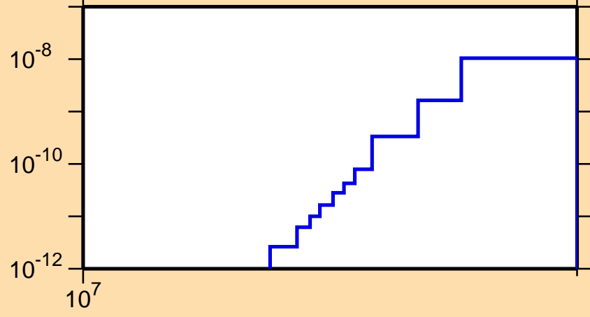
\sigma vs. E for ^{232}\text{Pu}(n,\text{He3})
