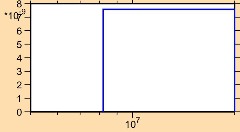
\sigma vs. E for ^{232}\text{Pu}(n,2n\alpha)
