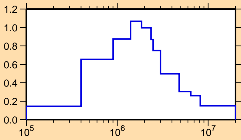
\sigma vs. E for ^{232}\text{Pu}(n,\text{inel.})
