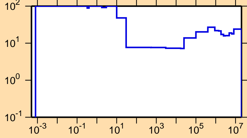
\Delta\sigma/\sigma vs. E for ^{232}\text{Pu}(n,\text{el.})
