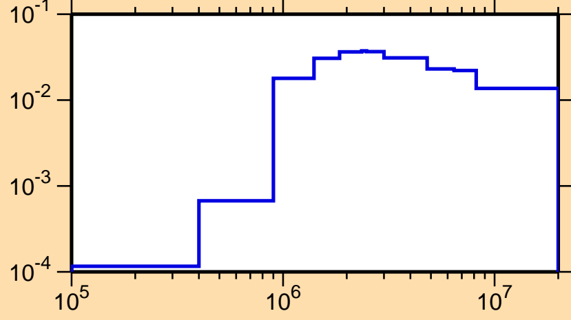
\sigma vs. E for ^{232}\text{Pu}(n,n\text{cont.})
