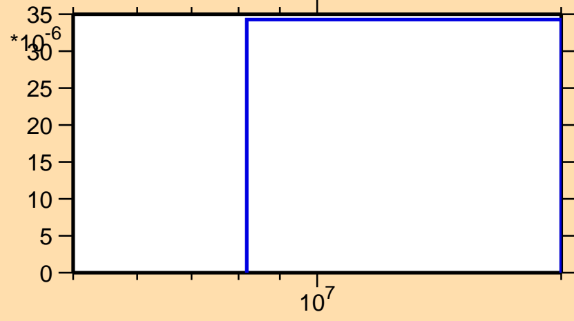
\sigma vs. E for ^{232}\text{Pu}(n,t)
