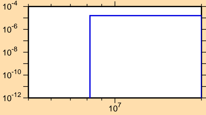
\sigma vs. E for ^{232}\text{Pu}(n,np)
