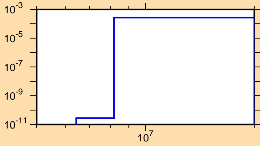
\sigma vs. E for ^{232}\text{Pu}(n,d)
