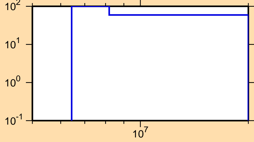
\Delta\sigma/\sigma vs. E for ^{232}\text{Pu}(n,2n)
