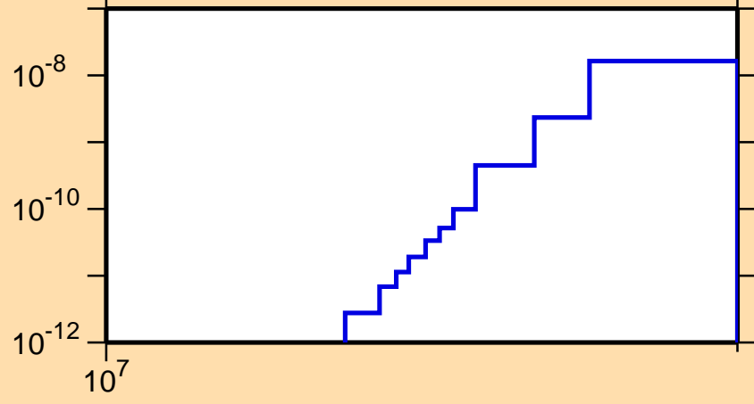
\sigma vs. E for ^{233}\text{Pu}(n,\text{He3})
