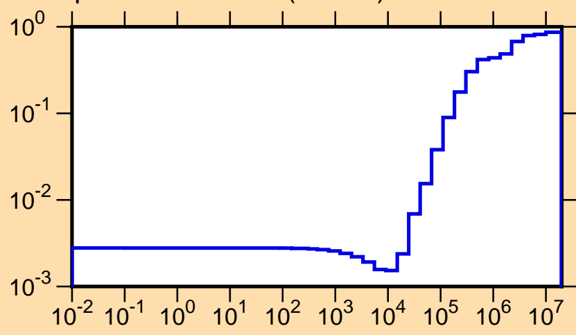
\mu vs. E for ^{233}\text{Pu}(\text{mt251})
