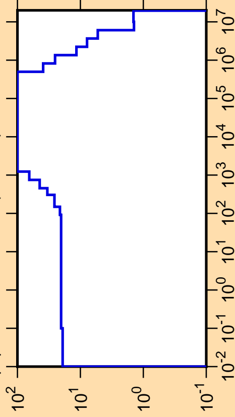
\Delta\mu/\mu vs. E for ^{233}\text{Pu}(\text{mt251})
