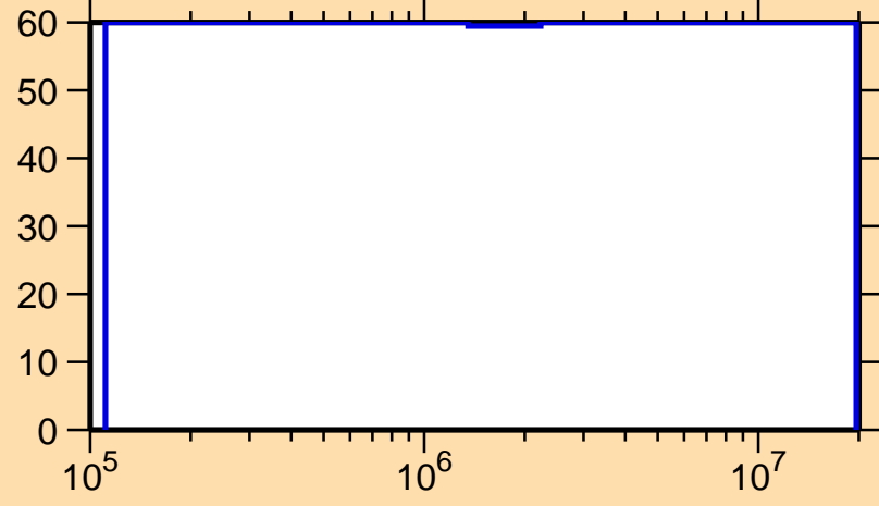
\Delta\sigma/\sigma vs. E for ^{233}\text{Pu}(n,ncont.)
