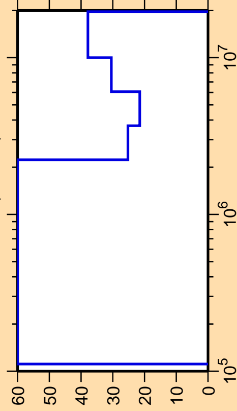
\Delta\sigma/\sigma vs. E for ^{233}\text{Pu}(n,\text{inel.})
