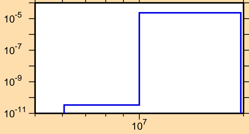
\sigma vs. E for ^{233}\text{Pu}(n,np)
