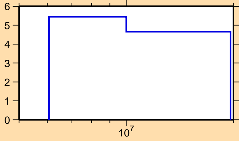
\Delta\sigma/\sigma vs. E for ^{233}\text{Pu}(n,\text{nonel.})
