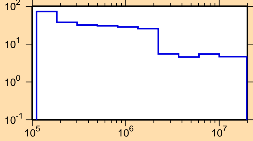
\Delta\sigma/\sigma vs. E for ^{233}\text{Pu}(n,\text{nonel.})
