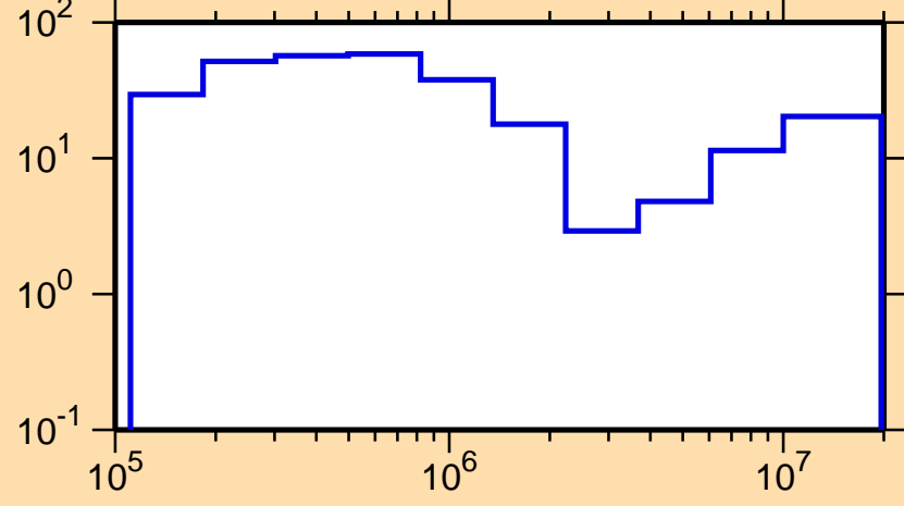
\Delta\sigma/\sigma vs. E for ^{233}\text{Pu}(n,\text{el.})
