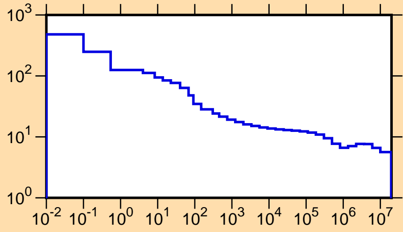
\sigma vs. E for ^{233}\text{Pu}(n,\text{tot.})
