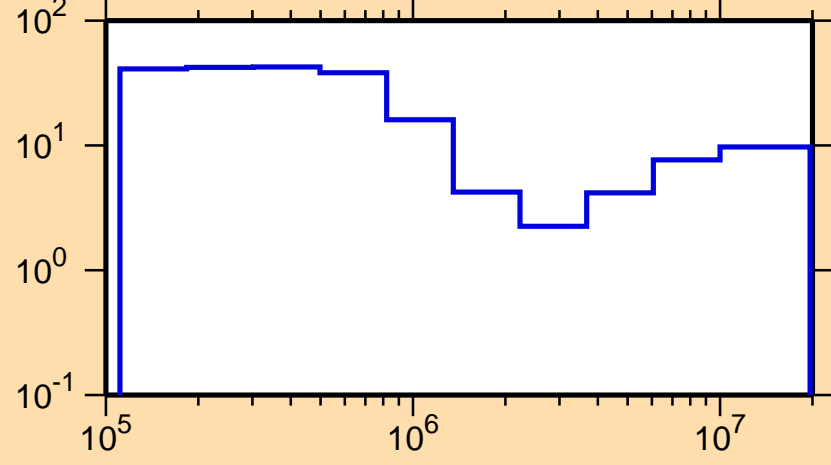
\Delta\sigma/\sigma vs. E for ^{233}\text{Pu}(n,\text{tot.})
