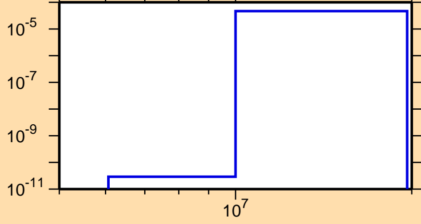
\sigma vs. E for ^{233}\text{Pu}(n,t)
