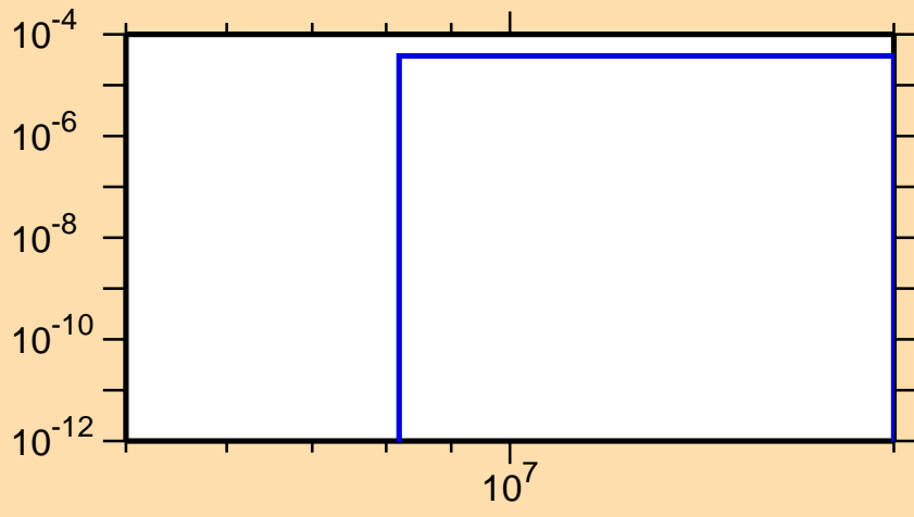
\sigma vs. E for ^{233}\text{Pu}(n,t)
