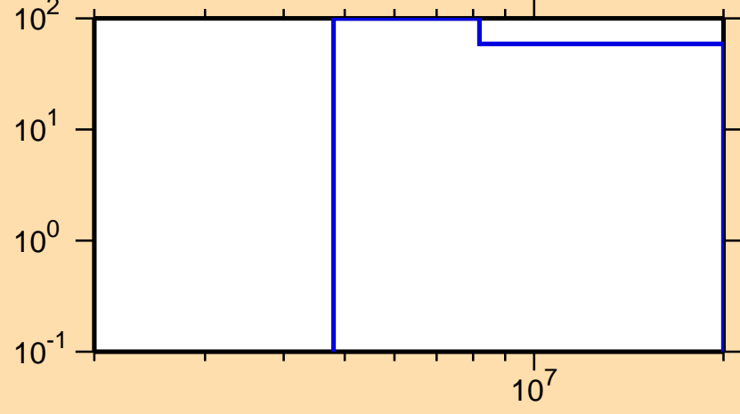
\Delta\sigma/\sigma vs. E for ^{233}\text{Pu}(n,2n)
