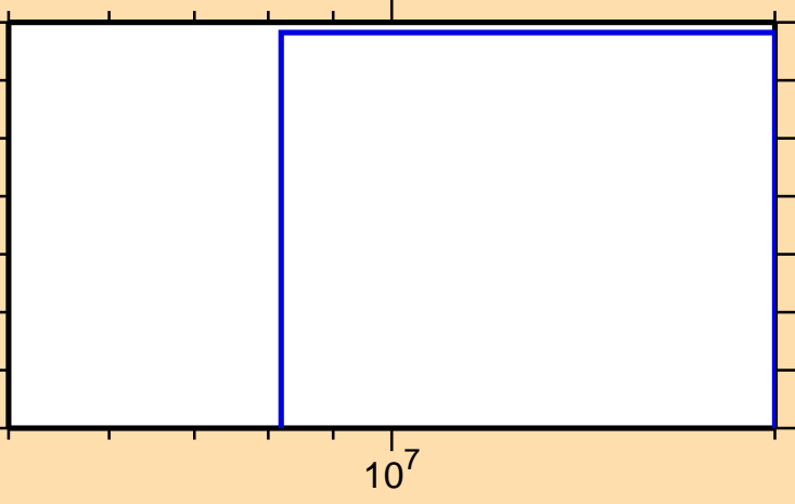
\sigma vs. E for ^{233}\text{Pu}(n,3n)
