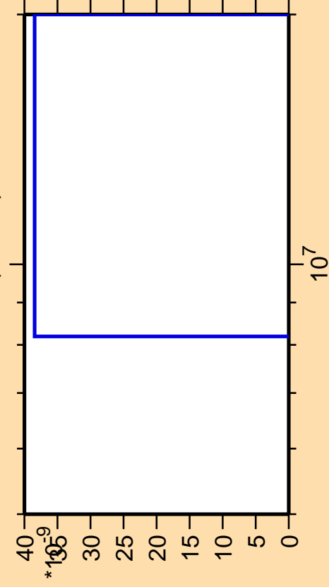
\Delta\sigma/\sigma vs. E for ^{233}\text{Pu} (mt 42)
