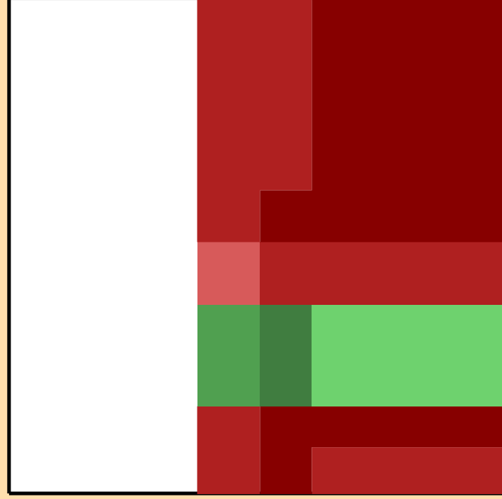
\Delta\sigma/\sigma vs. E for ^{233}\text{Pu}(n,2n)
