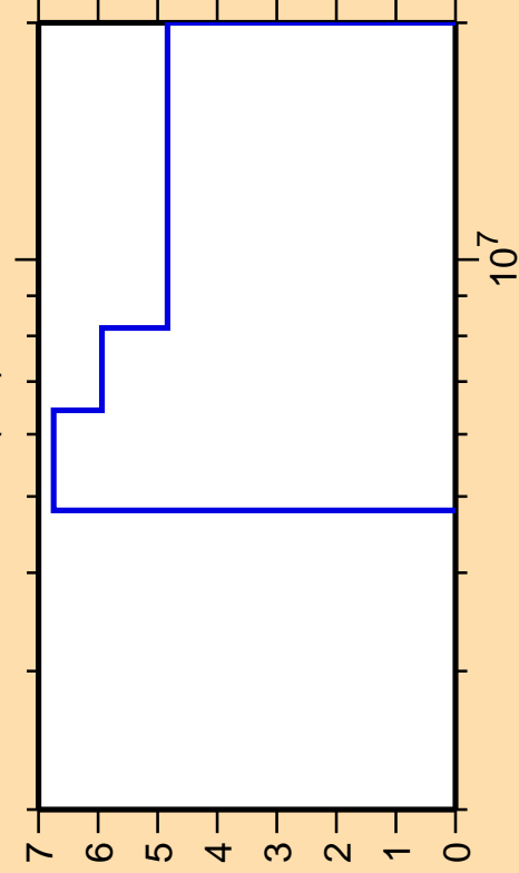
\Delta\sigma/\sigma vs. E for ^{233}\text{Pu}(n,f)
