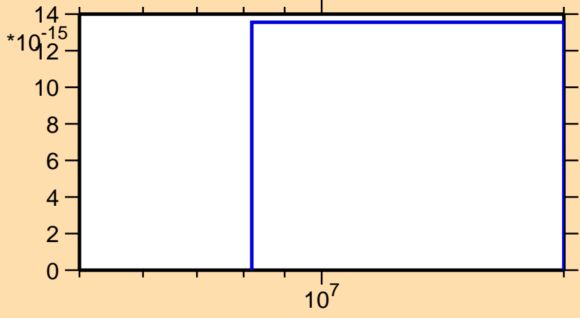
\sigma vs. E for ^{233}\text{Pu} (mt 34)
