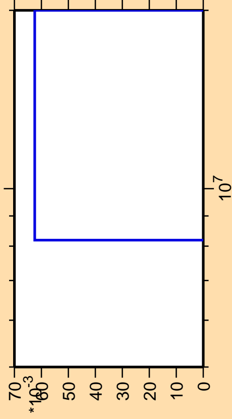
\Delta\sigma/\sigma vs. E for ^{233}\text{Pu} (mt 34)
