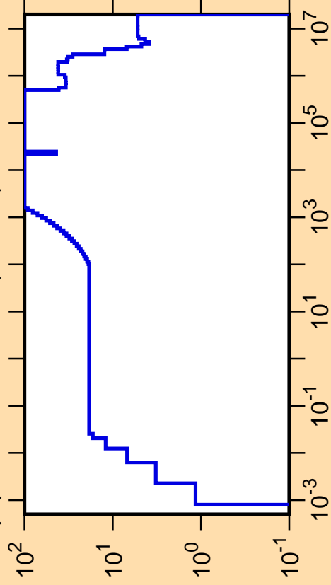
\Delta\mu/\mu vs. E for ^{234}\text{Pu}(\text{mt251})
