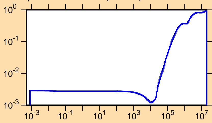
\mu vs. E for ^{234}\text{Pu}(\text{mt251})
