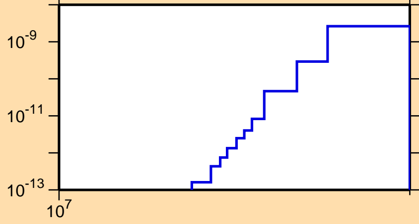
\sigma vs. E for ^{234}\text{Pu}(n,\text{He3})
