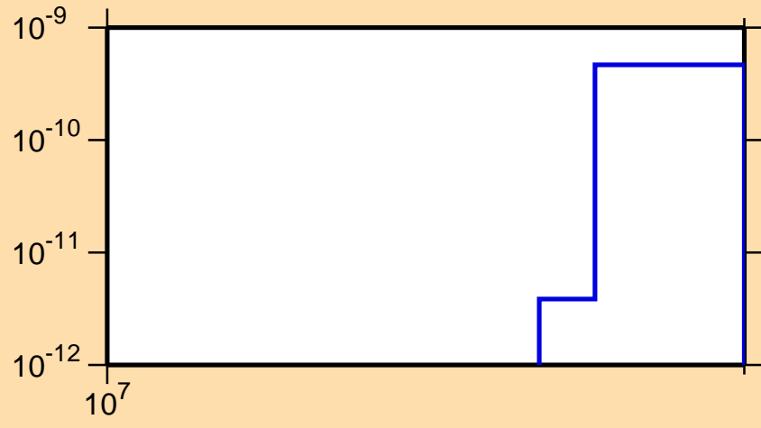
\sigma vs. E for ^{234}\text{Pu}(n,nt)
