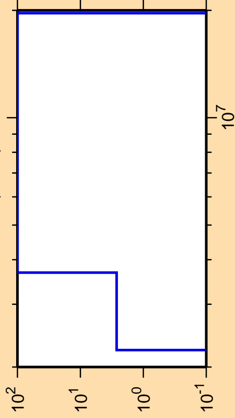
\Delta\sigma/\sigma vs. E for ^{234}\text{Pu}(n,n\alpha)
