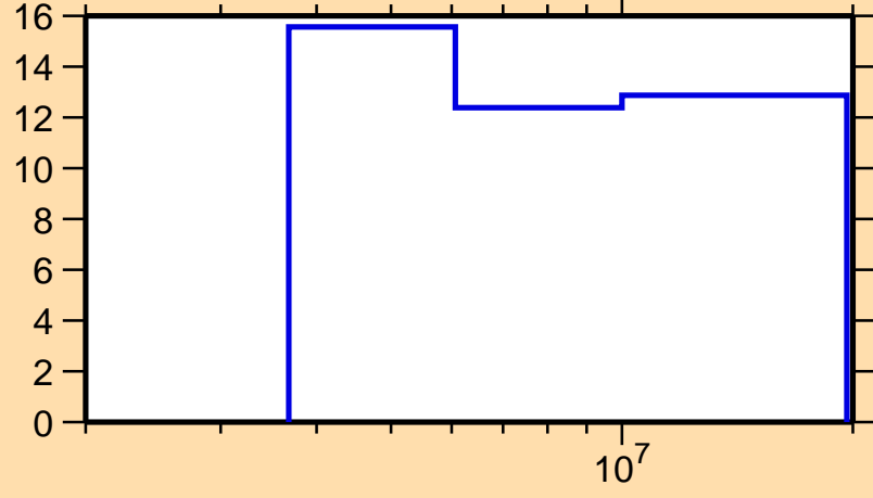
\Delta\sigma/\sigma vs. E for ^{234}\text{Pu}(n,n\text{nonel.})
