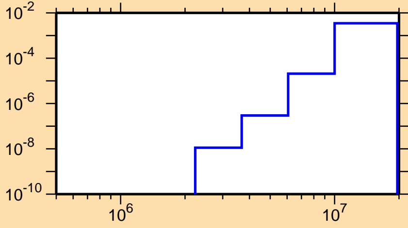
\sigma vs. E for ^{234}\text{Pu}(n,p)
