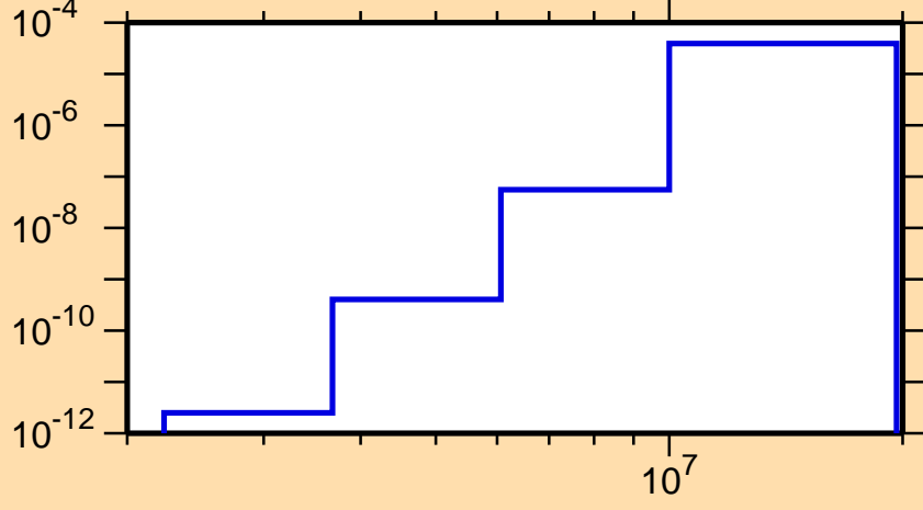
\sigma vs. E for ^{234}\text{Pu}(n,n\alpha)
