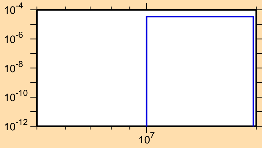
\sigma vs. E for ^{234}\text{Pu}(n,t)
