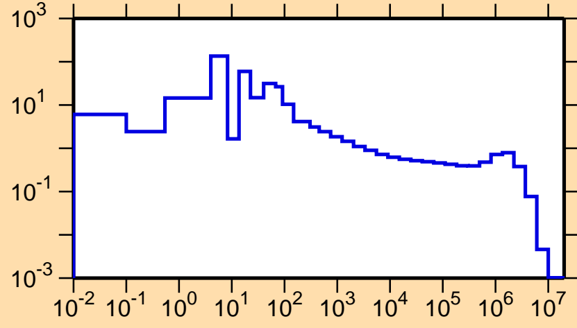
\sigma vs. E for ^{234}\text{Pu}(n,\gamma)
