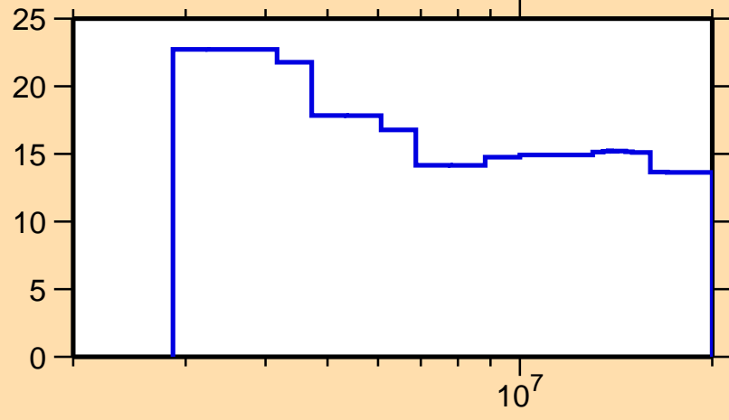
\Delta\sigma/\sigma vs. E for ^{235}\text{Pu}(n,\text{f})
