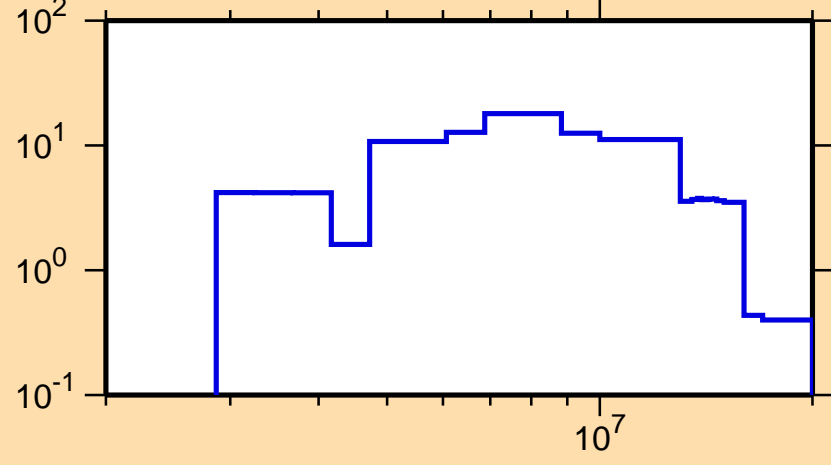
\Delta\sigma/\sigma vs. E for ^{235}\text{Pu}(n,\text{tot.})
