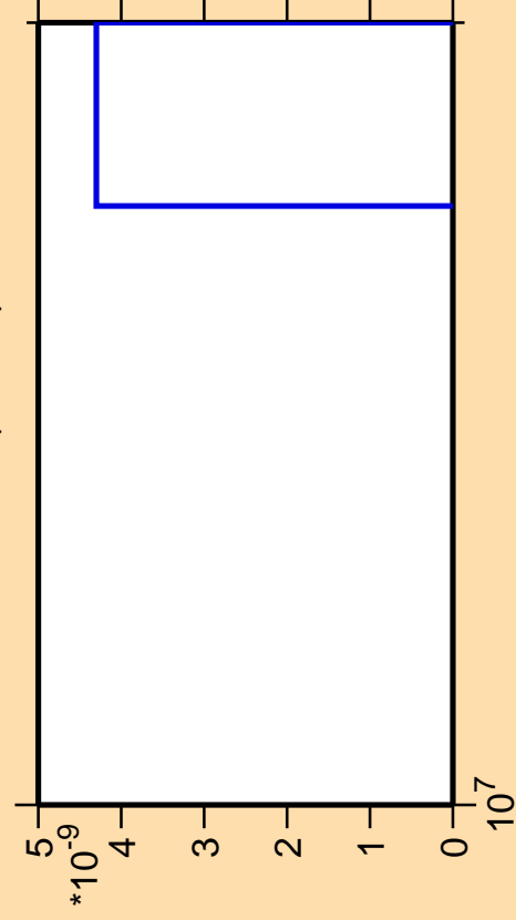
\Delta\sigma/\sigma vs. E for ^{235}\text{Pu} (mt 42)
