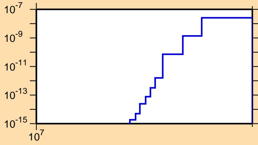
\sigma vs. E for ^{235}\text{Pu}(n,2np)
