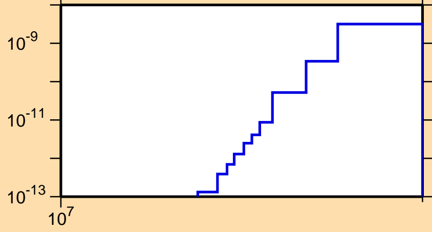
\sigma vs. E for ^{235}\text{Pu}(n,\text{He3})
