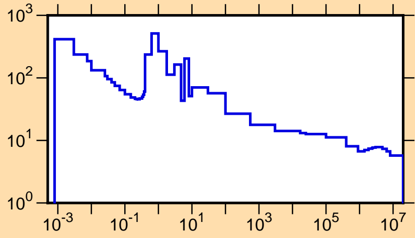
\sigma vs. E for ^{235}\text{Pu}(n,\text{tot.})
