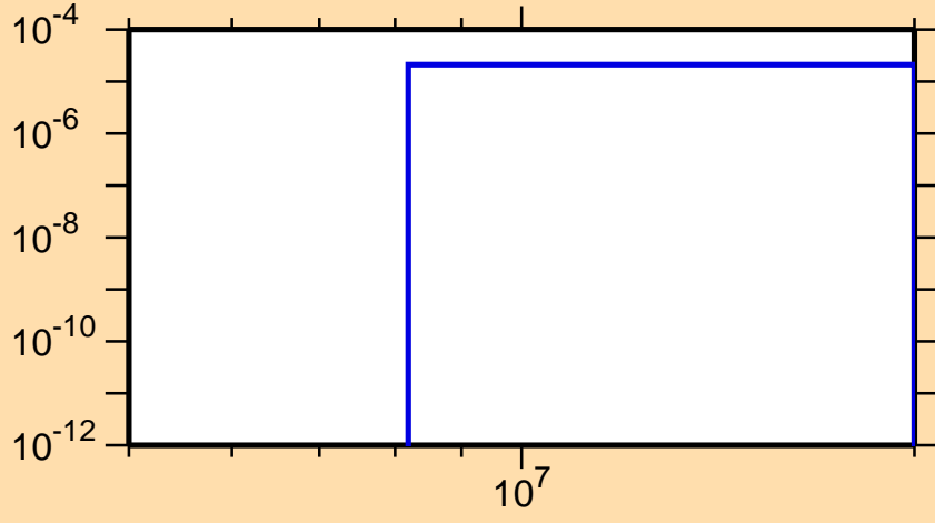
\sigma vs. E for ^{235}\text{Pu}(n,np)
