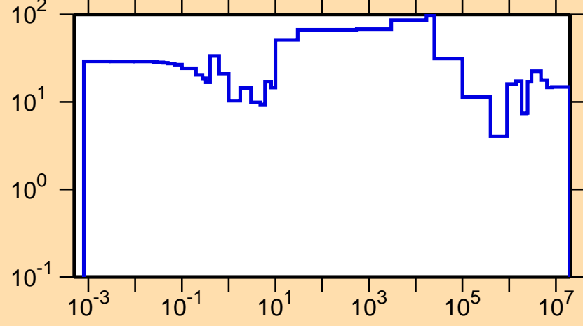
\Delta\sigma/\sigma vs. E for ^{235}\text{Pu}(n,f)
