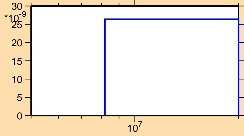
\sigma vs. E for ^{235}\text{Pu}(n,2n\alpha)
