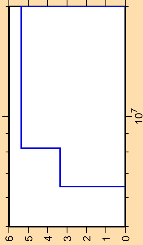
\Delta\sigma/\sigma vs. E for ^{235}\text{Pu}(n,d)
