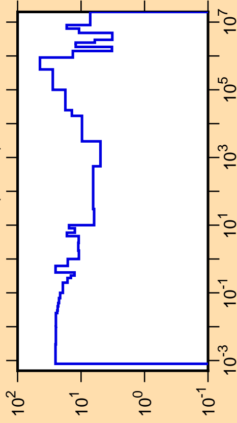
\Delta\sigma/\sigma vs. E for ^{235}\text{Pu}(n,\text{tot.})
