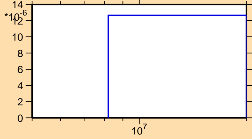
\sigma vs. E for ^{235}\text{Pu}(n,3n)
