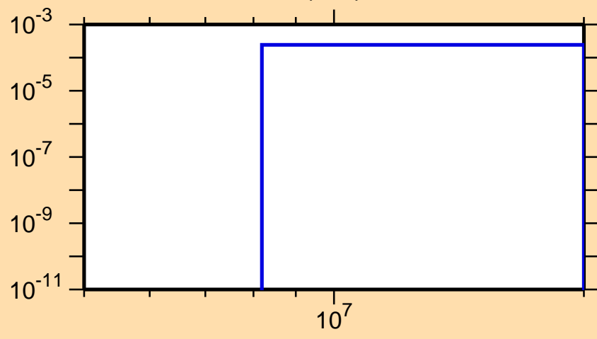
\sigma vs. E for ^{235}\text{Pu}(n,d)
