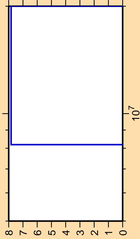
\Delta\sigma/\sigma vs. E for ^{235}\text{Pu}(n,t)
