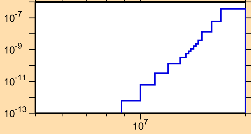
\sigma vs. E for ^{237}\text{Pu}(n,2n\alpha)
