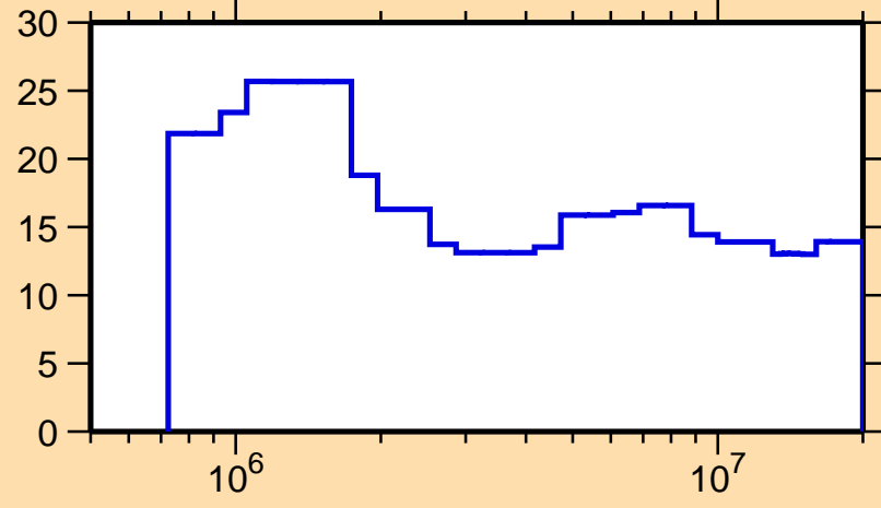
\Delta\sigma/\sigma vs. E for ^{237}\text{Pu}(n,n\text{onel.})
