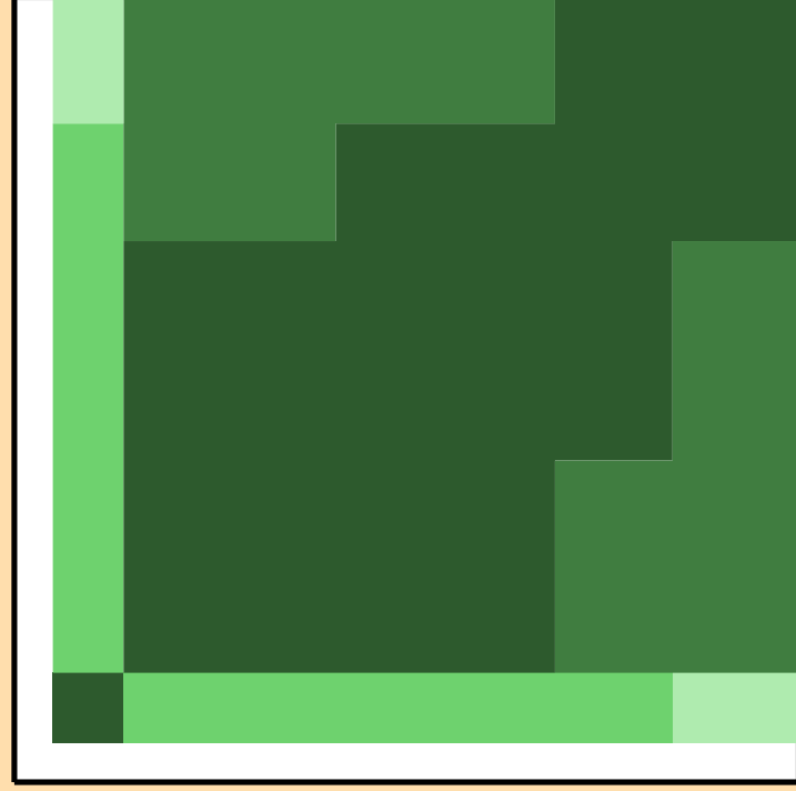
\sigma vs. E for ^{237}\text{Pu}(n,2n)
