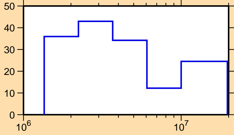
\Delta\sigma/\sigma vs. E for ^{237}\text{Pu}(n,el.)
