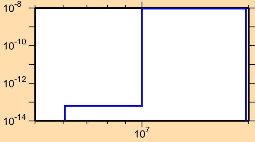
\sigma vs. E for ^{237}\text{Pu}(n,2n\alpha)
