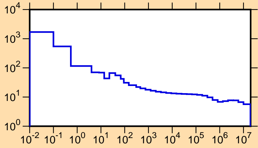
\sigma vs. E for ^{237}\text{Pu}(n,\text{tot.})
