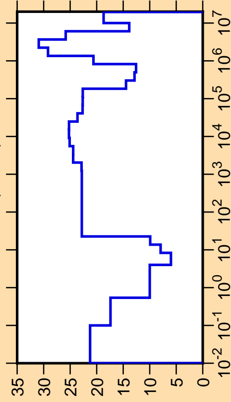
\Delta\sigma/\sigma vs. E for ^{237}\text{Pu}(n,\text{tot.})
