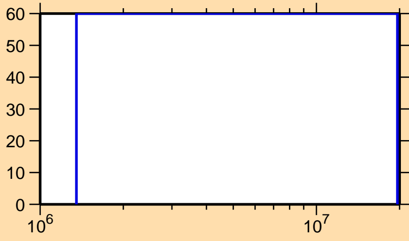
\Delta\sigma/\sigma vs. E for ^{237}\text{Pu}(n,\gamma)
