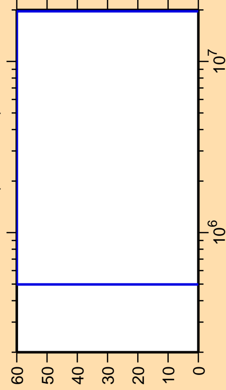
\Delta\sigma/\sigma vs. E for ^{237}\text{Pu}(n,\text{ncont.})
