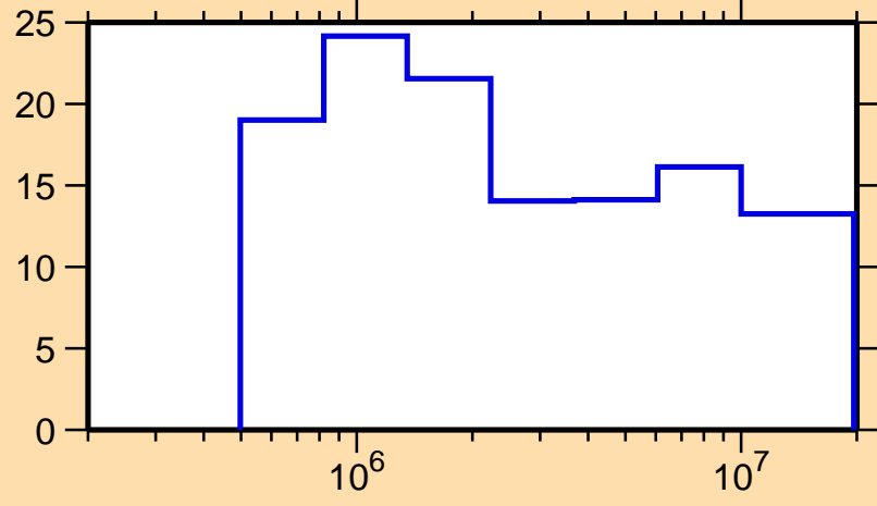
\Delta\sigma/\sigma vs. E for ^{237}\text{Pu}(n,n\text{nonel.})
