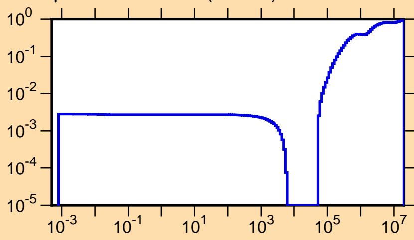
\mu vs. E for ^{238}\text{Pu}(\text{mt251})
