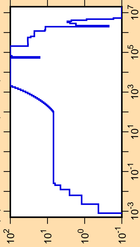
\Delta\mu/\mu vs. E for ^{238}\text{Pu}(\text{mt251})
