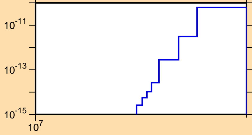
\sigma vs. E for ^{238}\text{Pu}(n,\text{He3})
