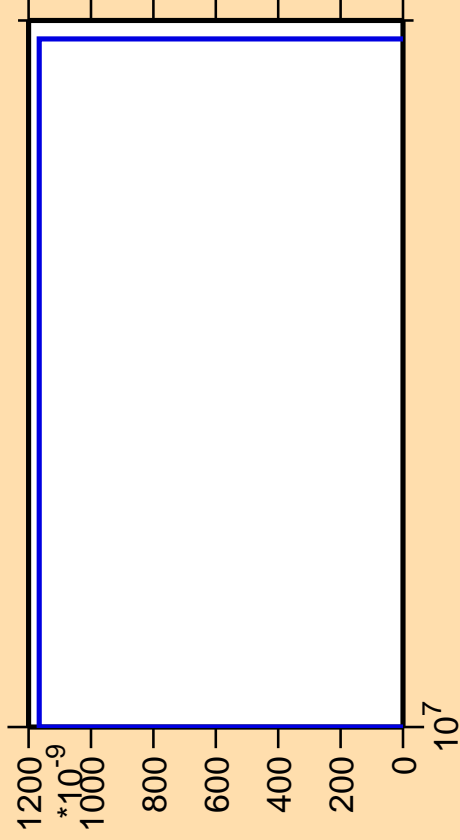
\Delta\sigma/\sigma vs. E for ^{238}\text{Pu} (mt 11)
