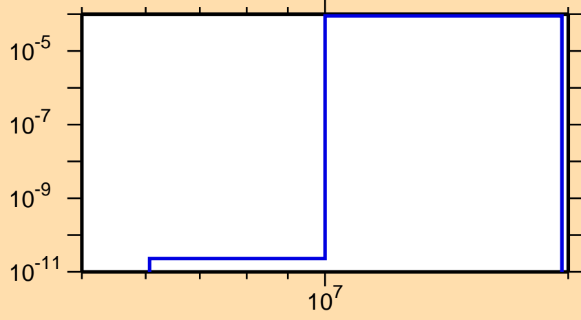
\sigma vs. E for ^{238}\text{Pu}(n,d)
