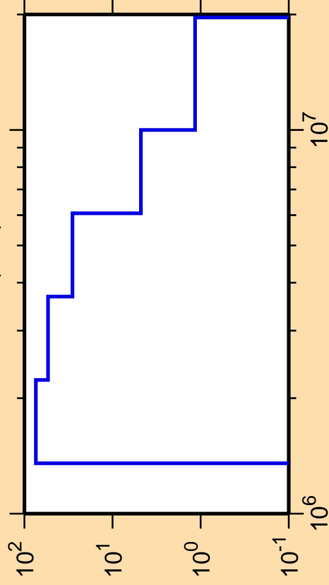
\Delta\sigma/\sigma vs. E for ^{238}\text{Pu}(n,\alpha)
