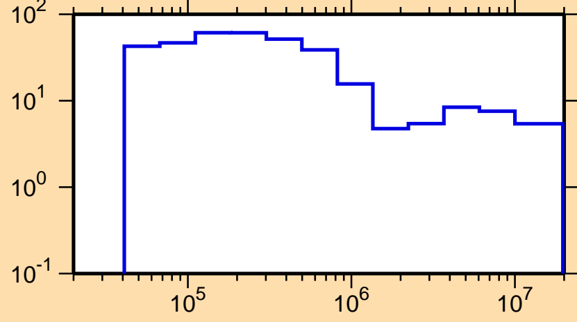
\Delta\sigma/\sigma vs. E for ^{238}\text{Pu}(n,\text{nonel.})
