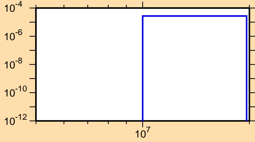
\sigma vs. E for ^{238}\text{Pu}(n,t)
