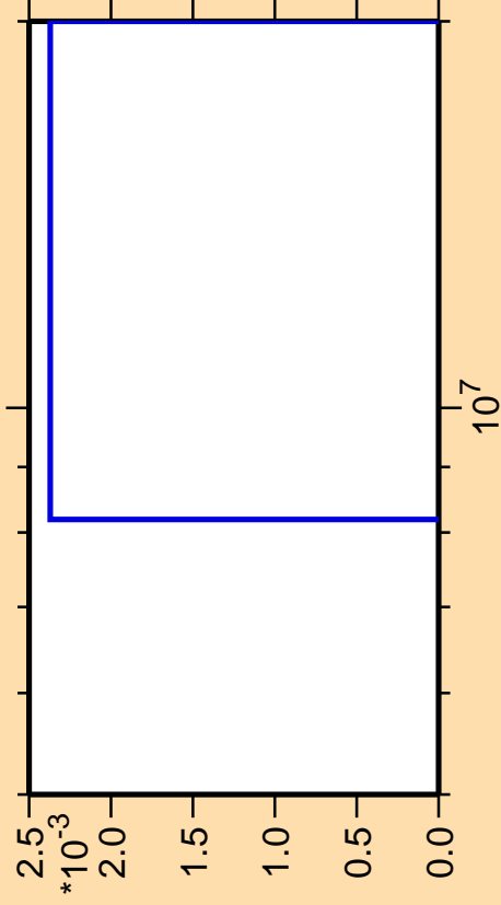
\Delta\sigma/\sigma vs. E for ^{238}\text{Pu}(n,p\alpha)
