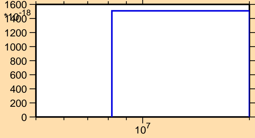
\sigma vs. E for ^{238}\text{Pu}(n,p\alpha)
