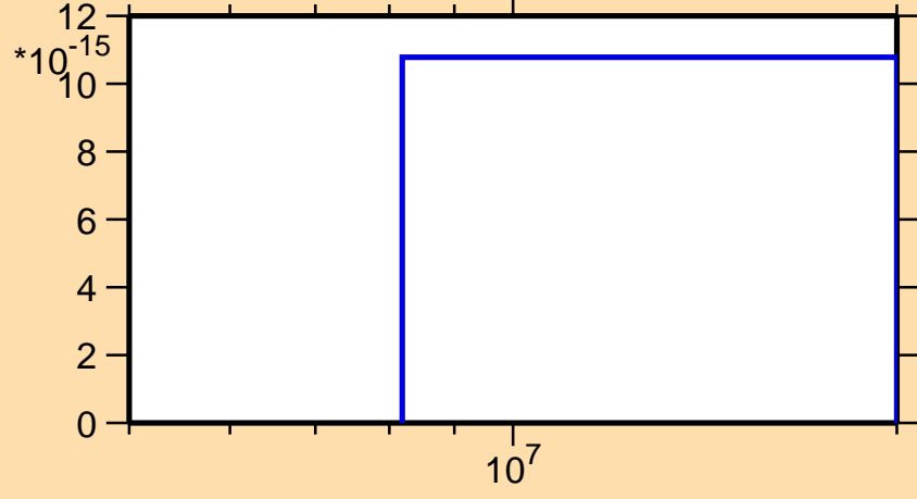
\sigma vs. E for ^{238}\text{Pu}(n,3n\alpha)
