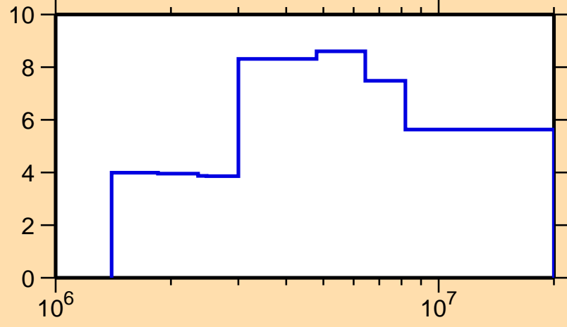
\Delta\sigma/\sigma vs. E for ^{238}\text{Pu}(n,n\text{onel.})
