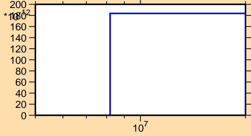
\sigma vs. E for ^{238}\text{Pu}(n,2np)
