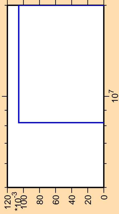
\Delta\sigma/\sigma vs. E for ^{238}\text{Pu}(n,\text{He3})
