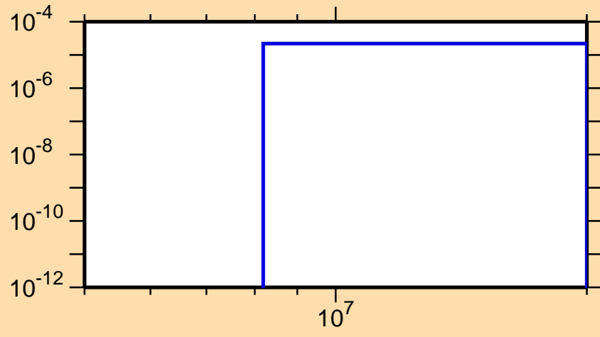
\sigma vs. E for ^{238}\text{Pu}(n,t)
