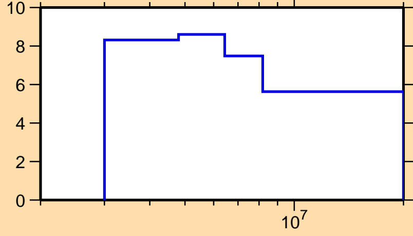
\Delta\sigma/\sigma vs. E for ^{238}\text{Pu}(n,\text{nonel.})
