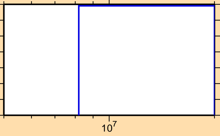
\sigma vs. E for ^{238}\text{Pu}(n,nt)
