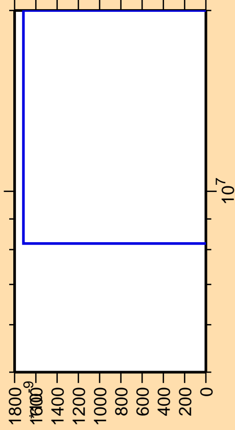
\Delta\sigma/\sigma vs. E for ^{238}\text{Pu}(\text{mt 11})
