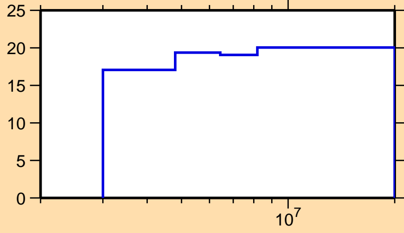
\Delta\sigma/\sigma vs. E for ^{238}\text{Pu}(n,el.)
