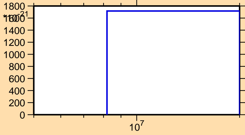
\sigma vs. E for ^{238}\text{Pu}(\text{mt 11})
