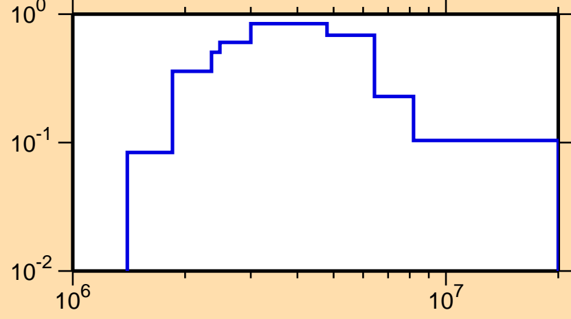
\sigma vs. E for ^{238}\text{Pu}(n,n\text{cont.})
