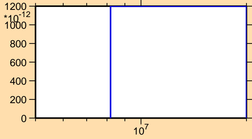
\sigma vs. E for ^{238}\text{Pu}(n,\text{nd})
