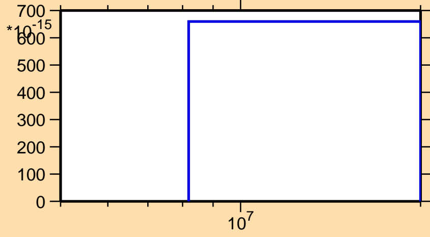
\sigma vs. E for ^{238}\text{Pu}(n,\text{He3})
