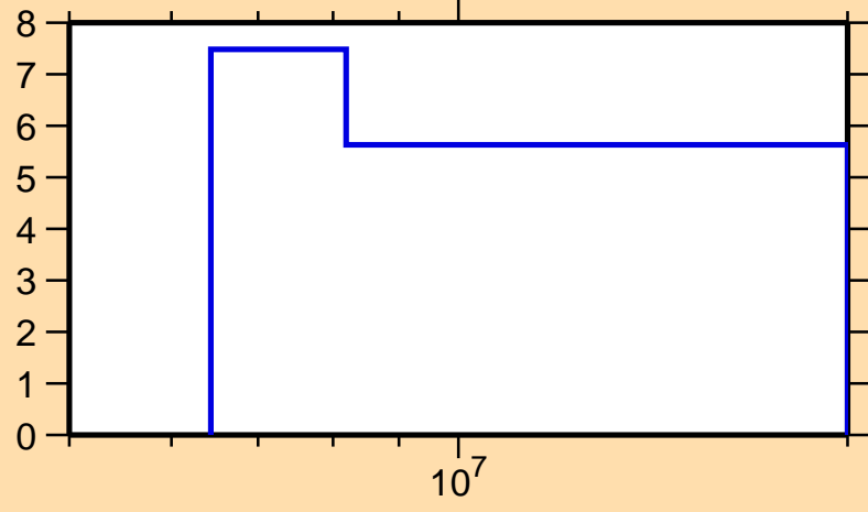
\Delta\sigma/\sigma vs. E for ^{238}\text{Pu}(n,\text{nonel.})
