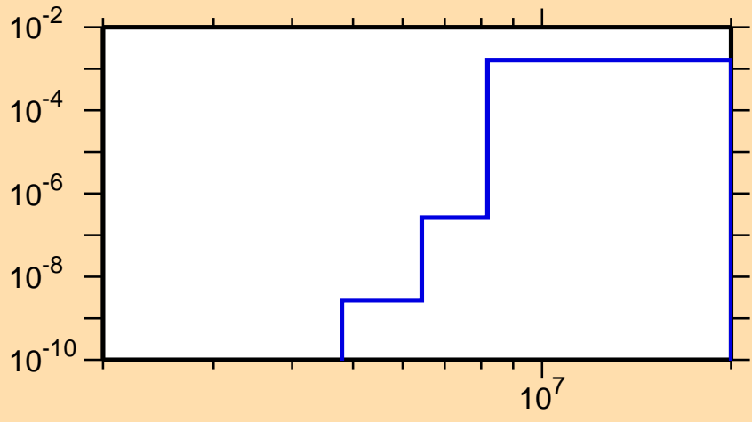
\sigma vs. E for ^{238}\text{Pu}(n,p)
