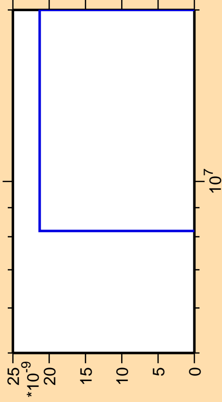
\Delta\sigma/\sigma vs. E for ^{238}\text{Pu} (mt 42)
