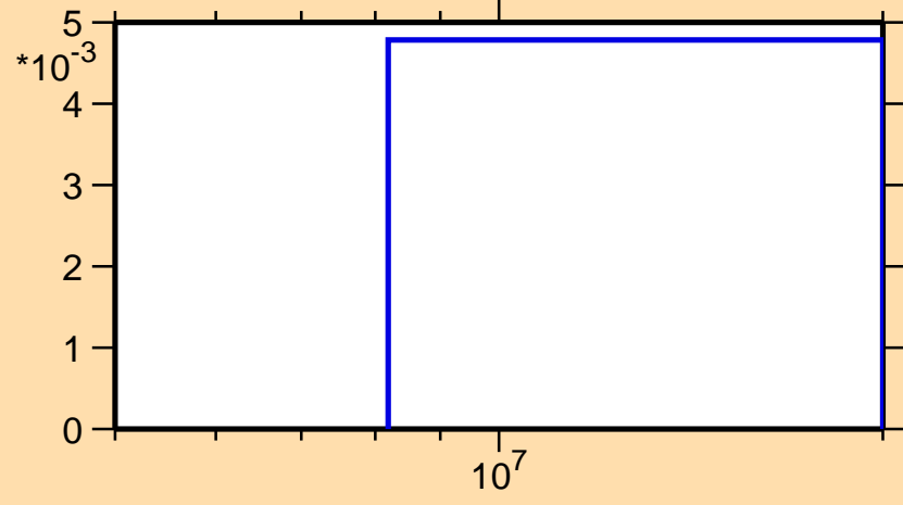
\sigma vs. E for ^{238}\text{Pu}(n,3n)
