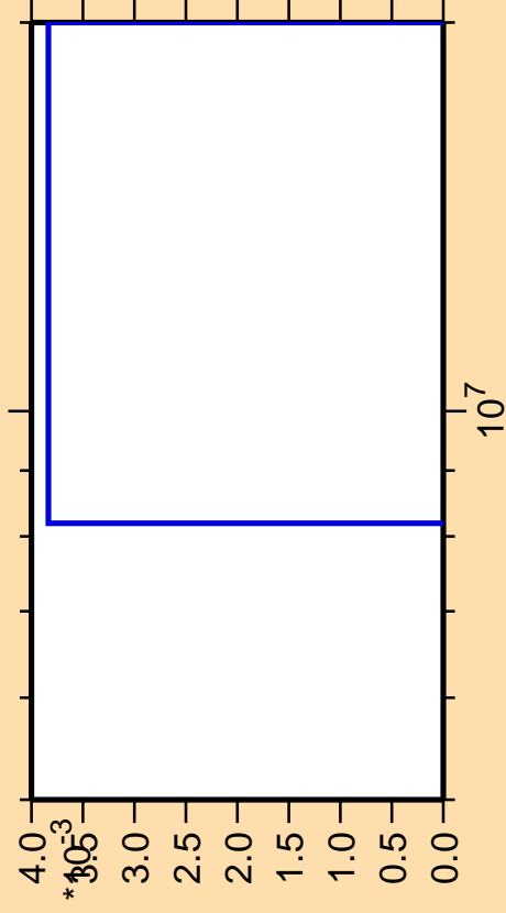
\Delta\sigma/\sigma vs. E for ^{238}\text{Pu}(n,3n\alpha)
