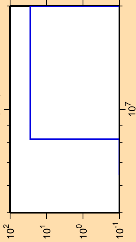
\Delta\sigma/\sigma vs. E for ^{238}\text{Pu}(n,d)
