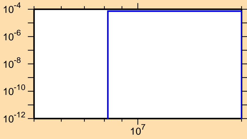
\sigma vs. E for ^{238}\text{Pu}(n,d)
