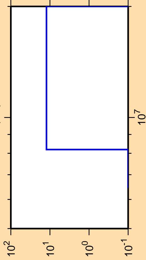
\Delta\sigma/\sigma vs. E for ^{238}\text{Pu}(n,t)
