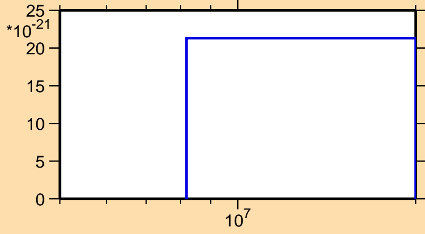
\sigma vs. E for ^{238}\text{Pu} (mt 42)
