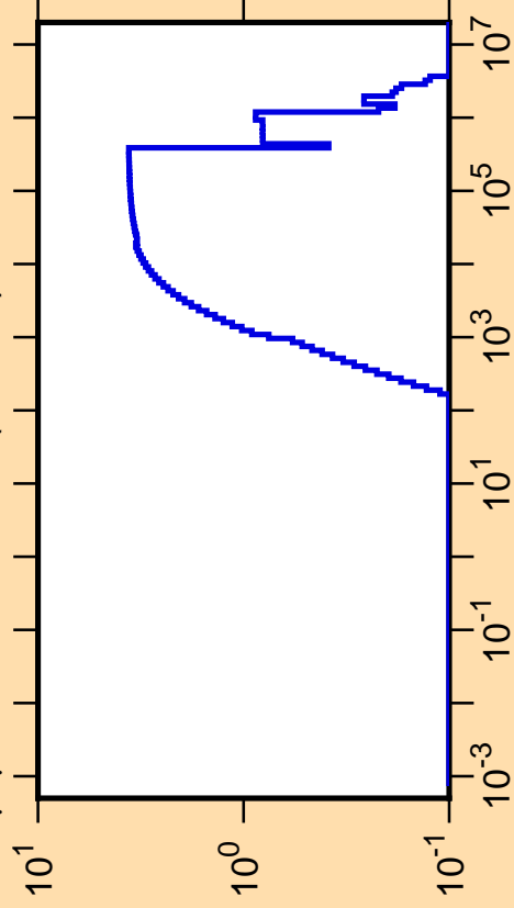
\Delta\mu/\mu vs. E for ^{240}\text{Pu}(\text{mt251})
