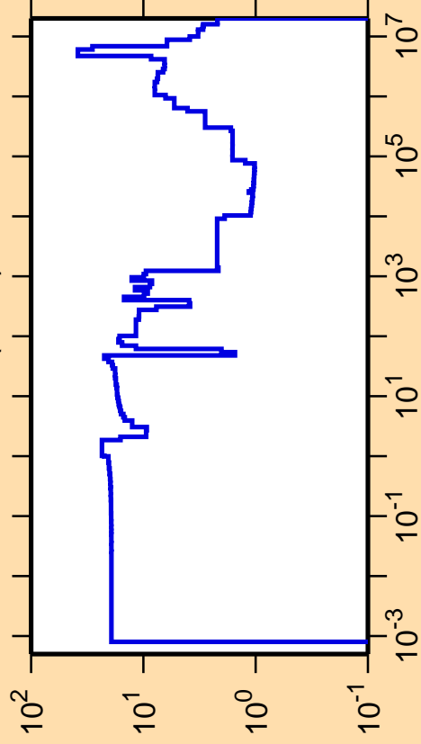
\Delta\sigma/\sigma vs. E for ^{242}\text{Pu}(n,\text{el.})
