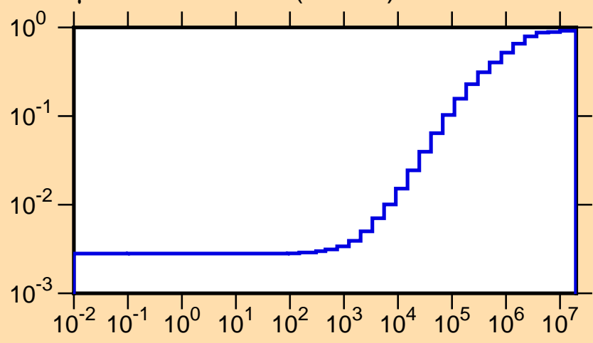
\mu vs. E for ^{242}\text{Pu}(\text{mt251})
