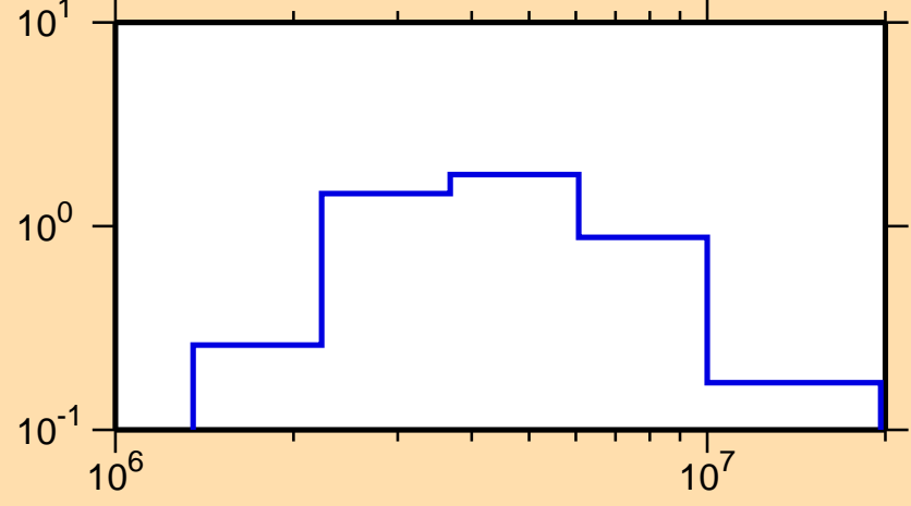
\sigma vs. E for ^{242}\text{Pu}(n,n\text{cont.})
