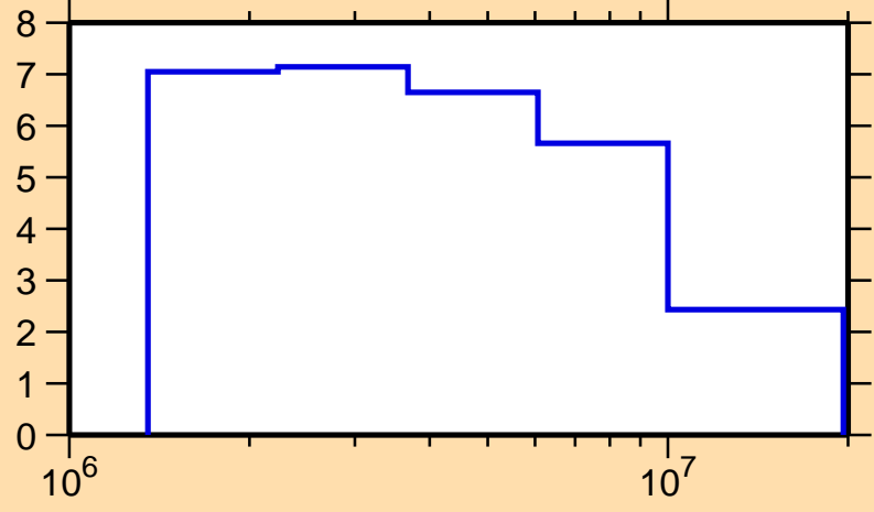
\Delta\sigma/\sigma vs. E for ^{242}\text{Pu}(n,n\text{onel.})
