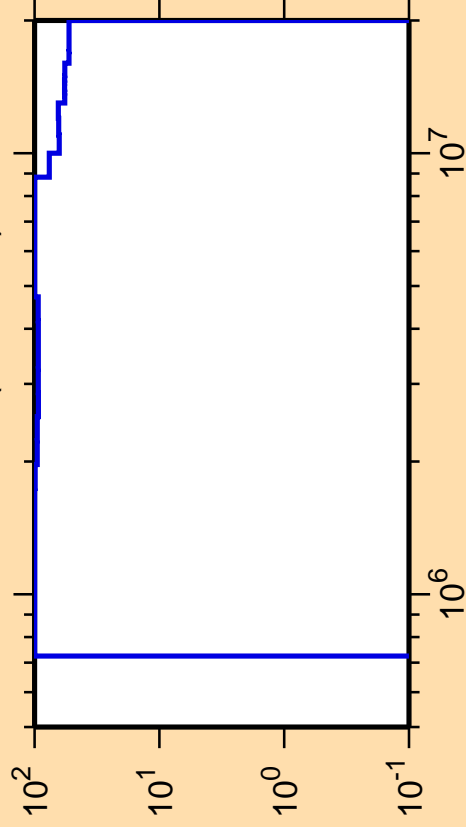
\Delta\sigma/\sigma vs. E for ^{243}\text{Pu}(n,\text{ncont.})
