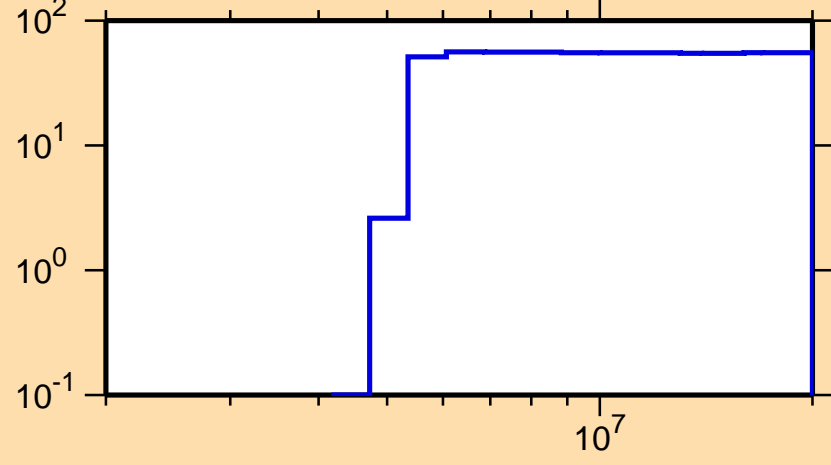
\Delta\sigma/\sigma vs. E for ^{243}\text{Pu}(n,p)
