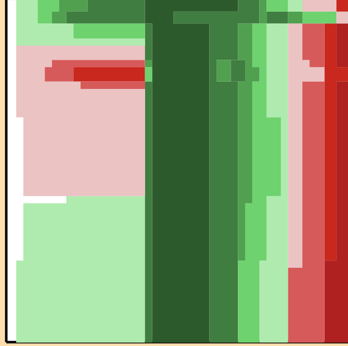
\Delta\sigma/\sigma vs. E for ^{243}\text{Pu}(n,n_1)
