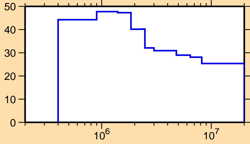
\Delta\sigma/\sigma vs. E for ^{243}\text{Pu}(n,n\text{onel.})
