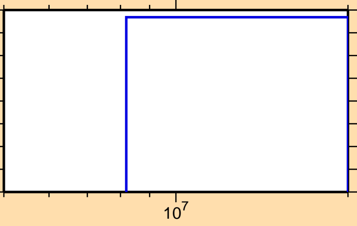
\sigma vs. E for ^{243}\text{Pu}(n,\text{nd})
