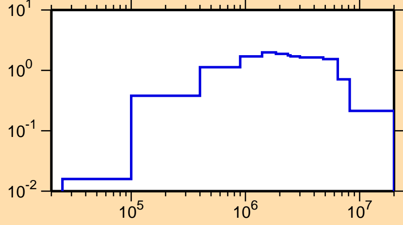
\sigma vs. E for ^{243}\text{Pu}(n,\text{inel.})
