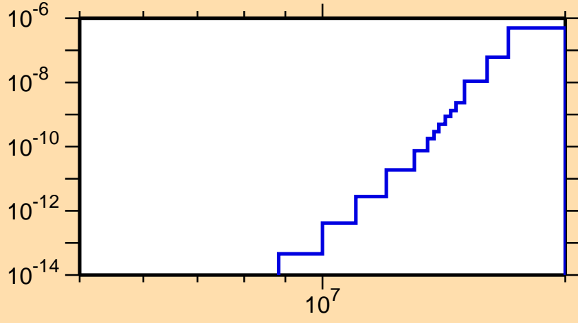
\sigma vs. E for ^{245}\text{Pu}(n,2n\alpha)
