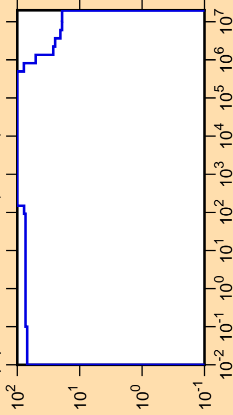
\Delta\mu/\mu vs. E for ^{245}\text{Pu}(\text{mt251})
