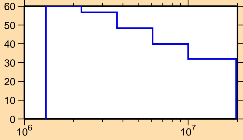
\Delta\sigma/\sigma vs. E for ^{245}\text{Pu}(n,n\text{onel.})
