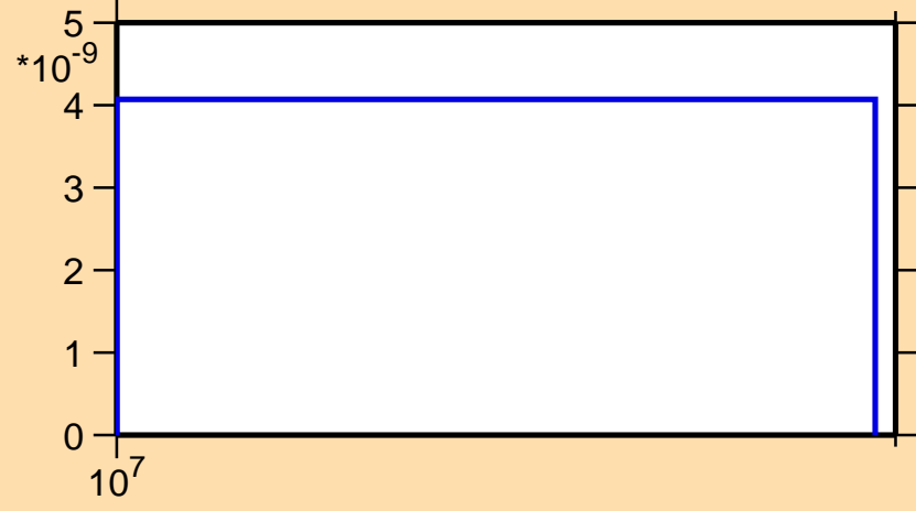
\sigma vs. E for ^{245}\text{Pu}(n,\text{nd})
