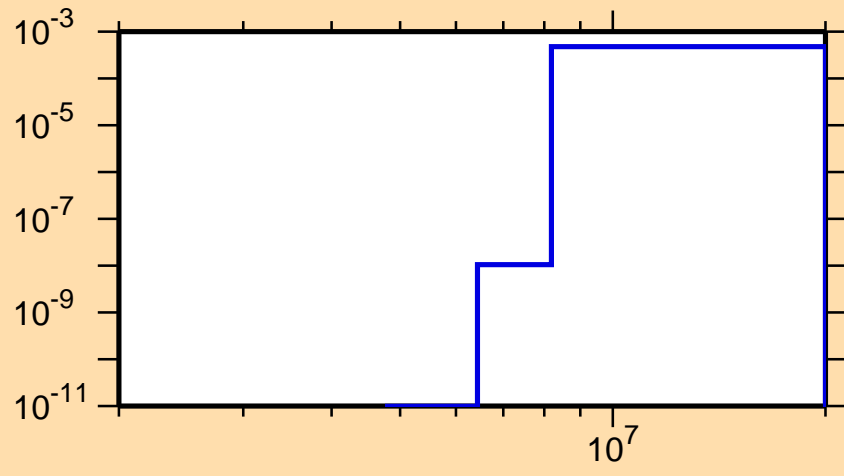
\sigma vs. E for ^{245}\text{Pu}(n,p)
