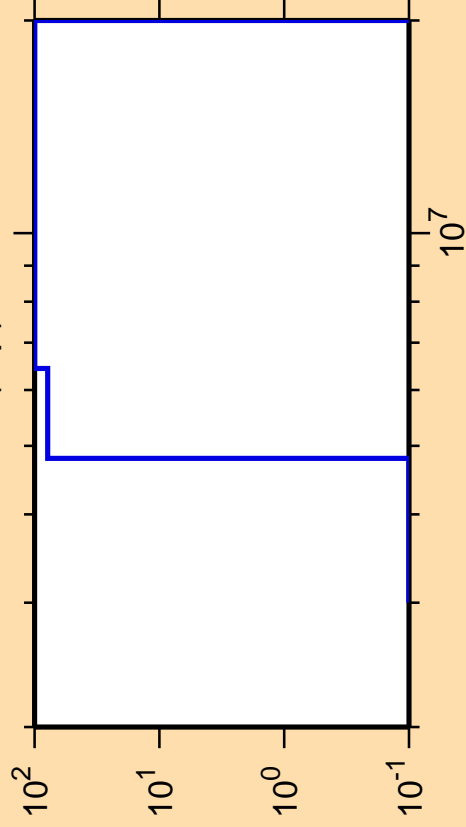
\Delta\sigma/\sigma vs. E for ^{245}\text{Pu}(n,p)
