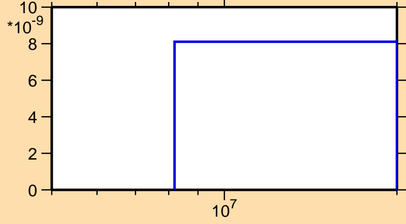
\sigma vs. E for ^{245}\text{Pu}(n,2n\alpha)
