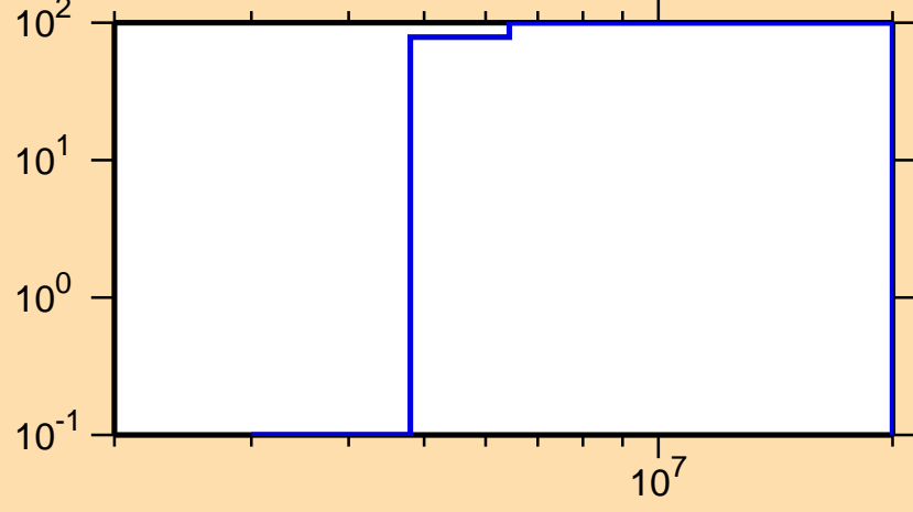
\Delta\sigma/\sigma vs. E for ^{245}\text{Pu}(n,p)
