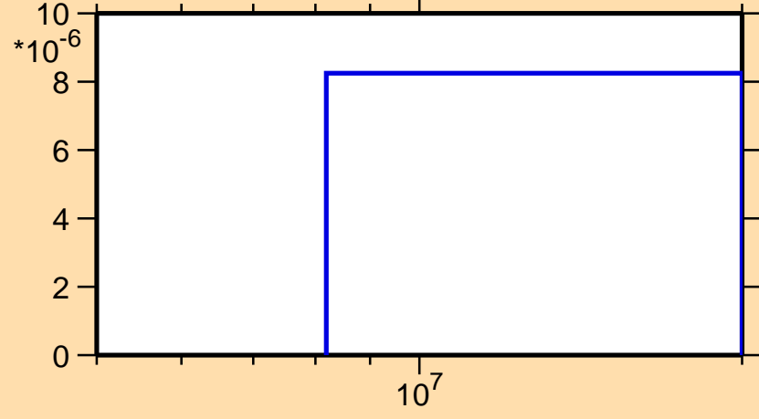
\sigma vs. E for ^{245}\text{Pu}(n,np)
