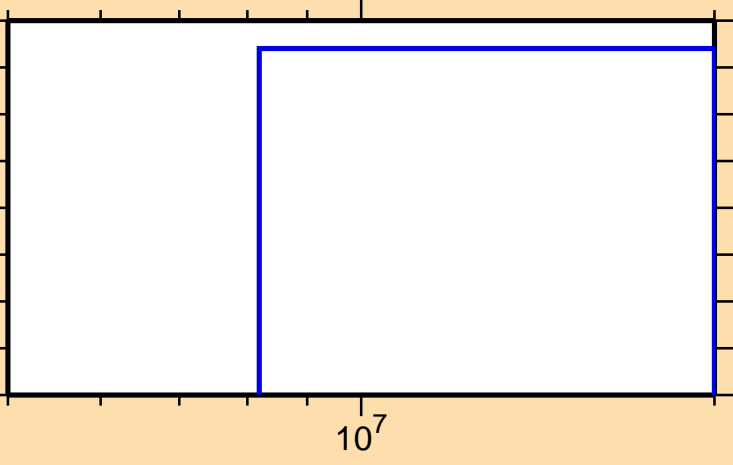
\sigma vs. E for ^{245}\text{Pu}(n,\text{nd})
