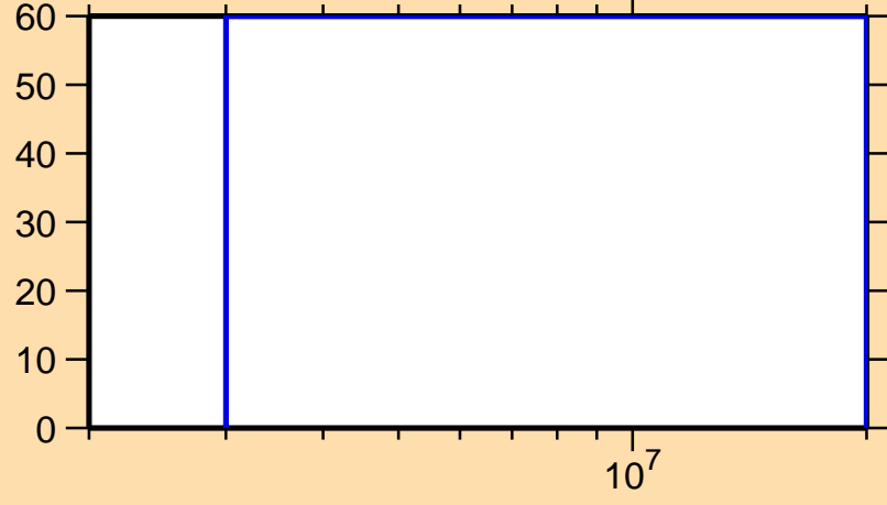
\Delta\sigma/\sigma vs. E for ^{245}\text{Pu}(n,n\text{cont.})
