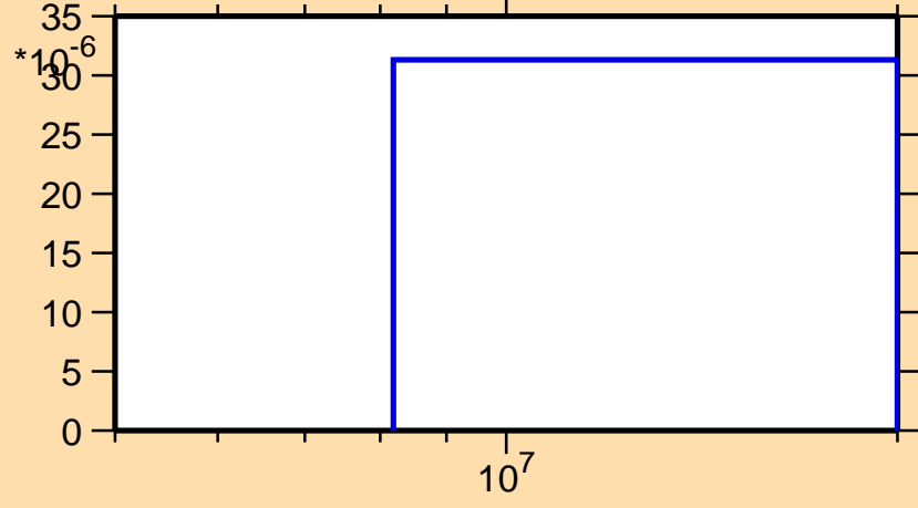
\sigma vs. E for ^{245}\text{Pu}(n,d)
