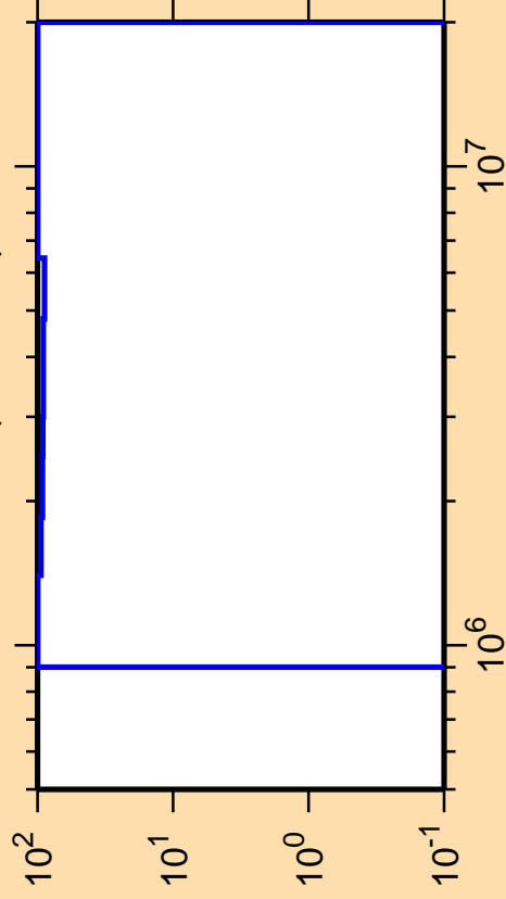
\Delta\sigma/\sigma vs. E for ^{245}\text{Pu}(n,\text{ncont.})
