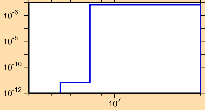
\sigma vs. E for ^{245}\text{Pu}(n,n\alpha)
