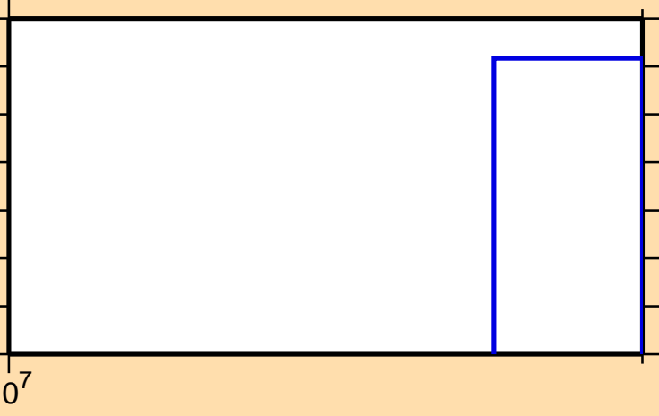
\sigma vs. E for ^{246}\text{Pu}(\text{mt } 42)
