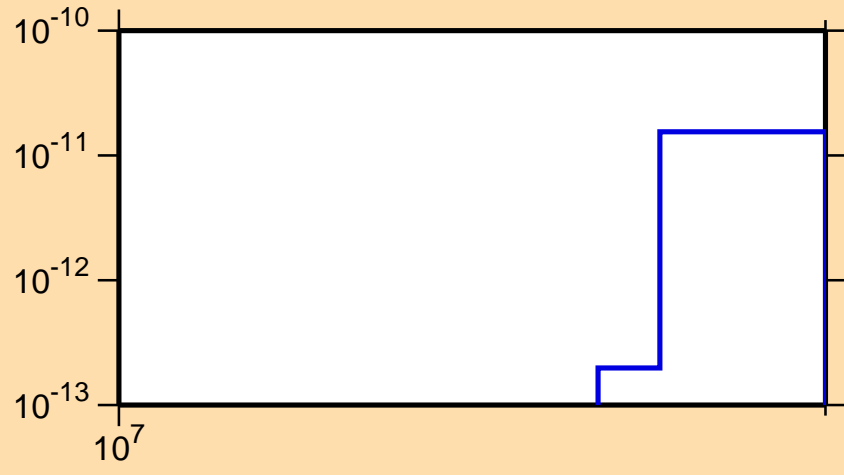
\sigma vs. E for ^{246}\text{Pu}(n,3n\alpha)
