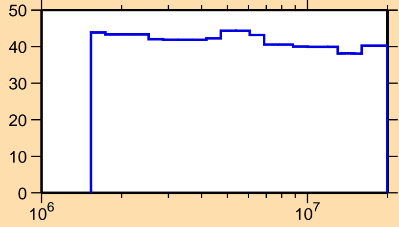
\Delta\sigma/\sigma vs. E for ^{246}\text{Pu}(n,n\text{nonel.})
