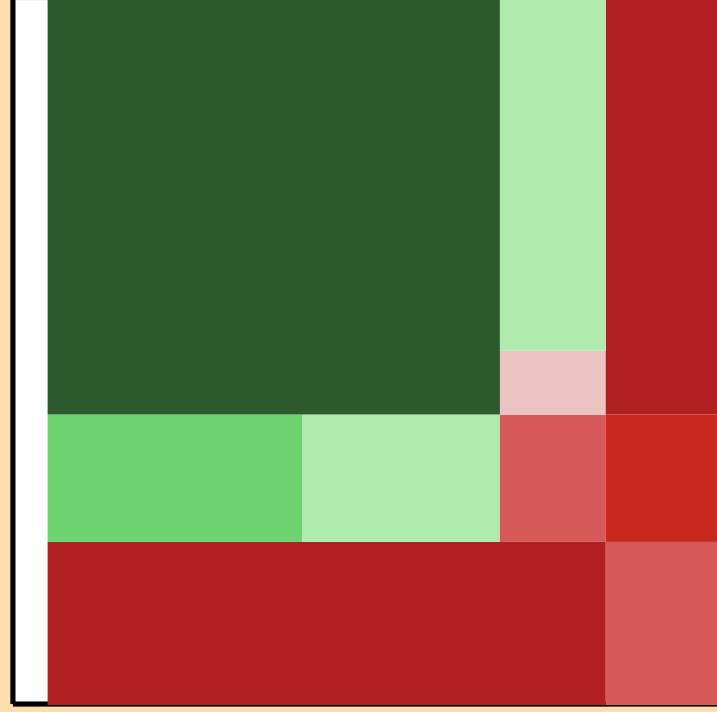
\Delta\sigma/\sigma vs. E for ^{246}\text{Pu}(n,2n)
