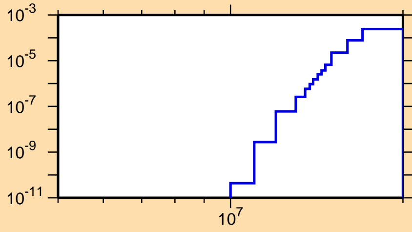
\sigma vs. E for ^{246}\text{Pu}(n,t)
