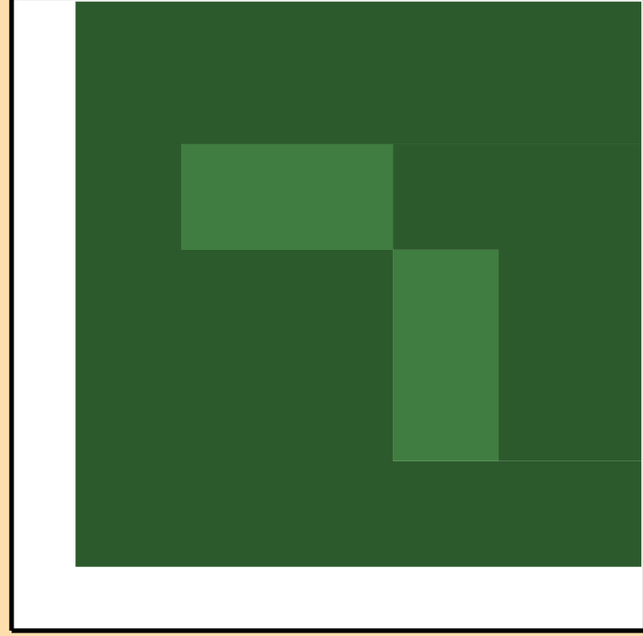
\sigma vs. E for ^{246}\text{Pu}(n,n\text{cont.})
