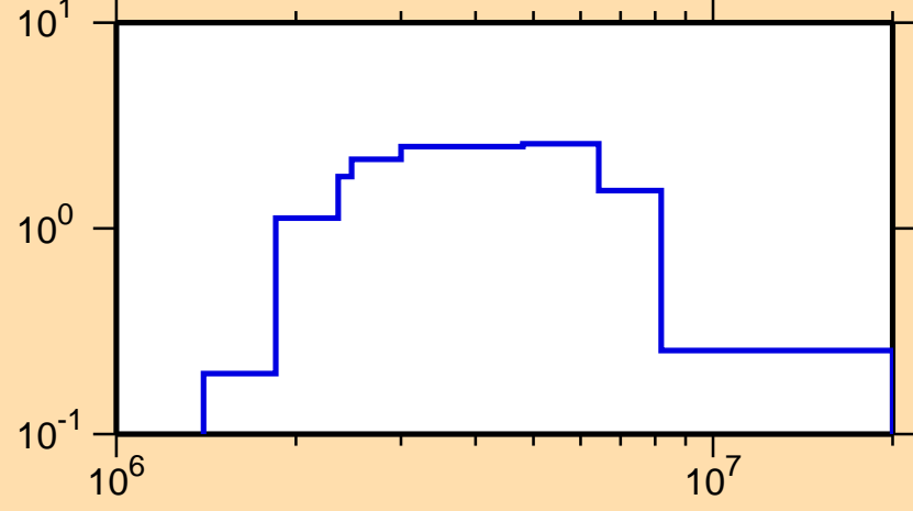
\sigma vs. E for ^{246}\text{Pu}(n,n\text{cont.})
