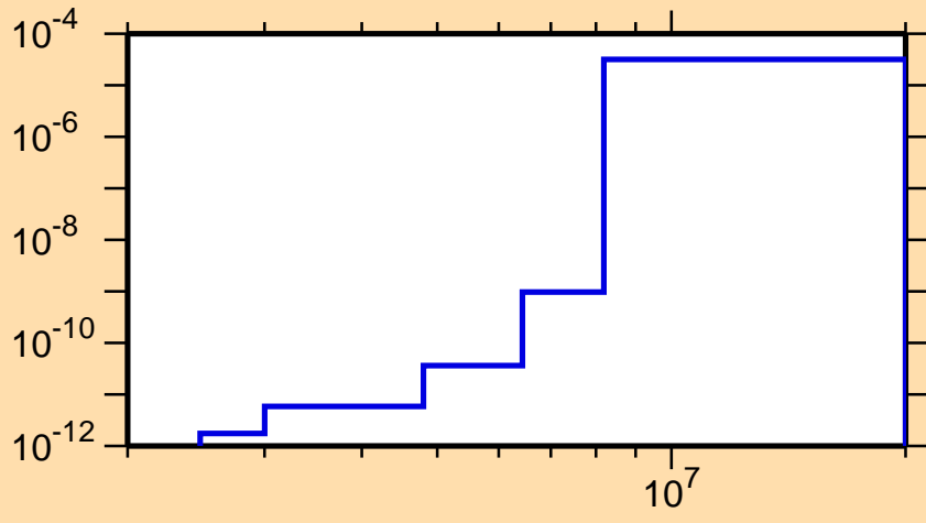
\sigma vs. E for ^{246}\text{Pu}(n,\alpha)
