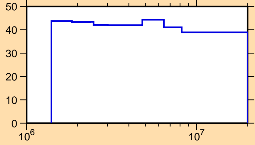
\Delta\sigma/\sigma vs. E for ^{246}\text{Pu}(n,n\text{onel.})
