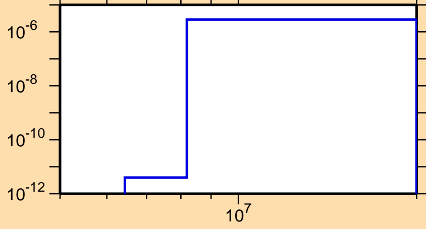
\sigma vs. E for ^{246}\text{Pu}(n,n\alpha)
