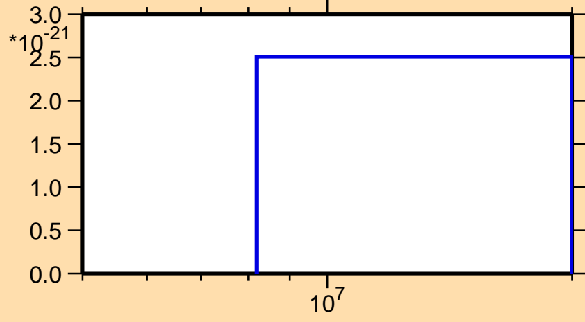
\sigma vs. E for ^{246}\text{Pu}(\text{mt } 42)
