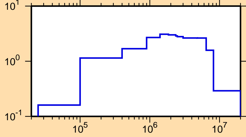
\sigma vs. E for ^{246}\text{Pu}(n,\text{inel.})
