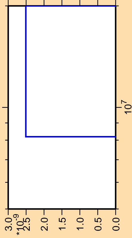
\Delta\sigma/\sigma vs. E for ^{246}\text{Pu}(\text{mt } 42)
