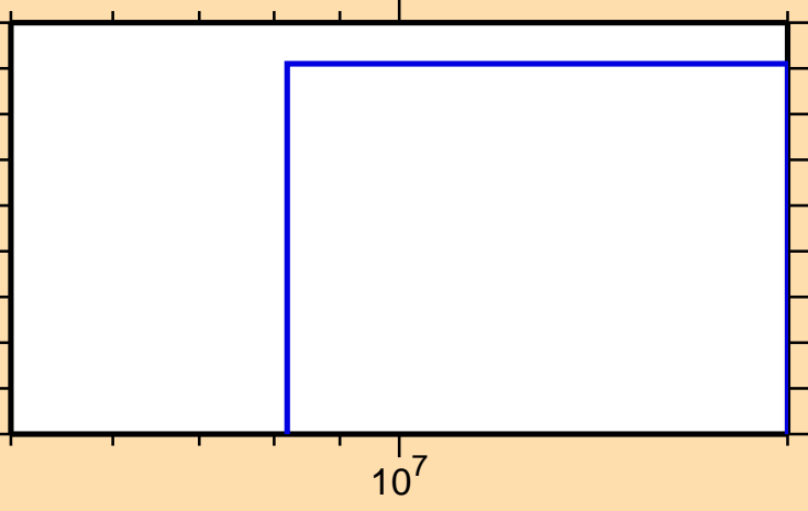
\sigma vs. E for ^{246}\text{Pu}(n,np)
